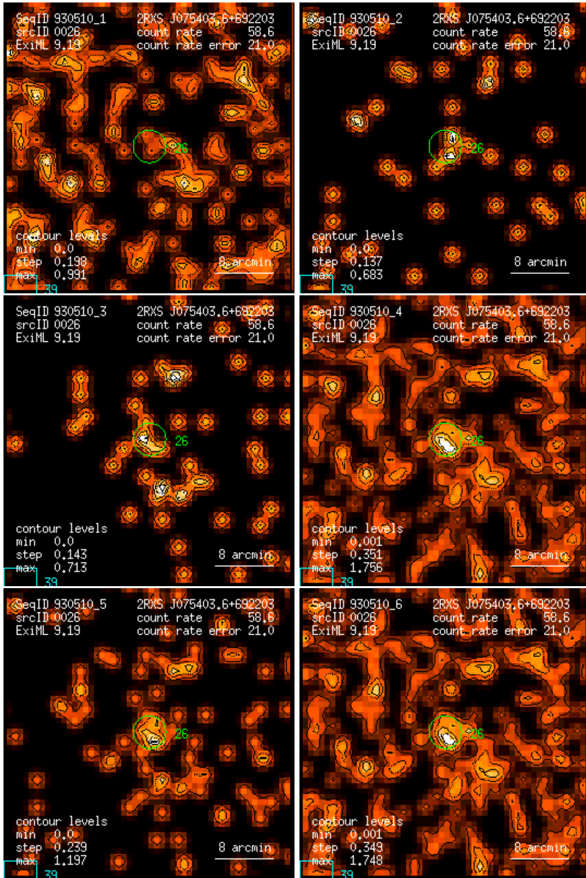
Figure 26: RASS 930510: detection 0026: band rate images, Gaussian filter: (1) PSPC channels 11 – 41, (2) 52 – 90, (3) 91 – 201, (4) 11 – 235, (5) 52 – 201, (6) 11 – 201. Broad band rates in counts/ks. Band rate contour levels in counts/ks/arcmin 2 .
