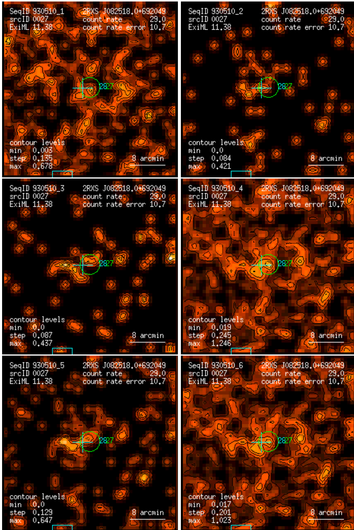
Figure 27: RASS 930510: detection 0027: band rate images, Gaussian filter: (1) PSPC channels 11 – 41, (2) 52 – 90, (3) 91 – 201, (4) 11 – 235, (5) 52 – 201, (6) 11 – 201. Broad band rates in counts/ks. Band rate contour levels in counts/ks/arcmin 2 .
