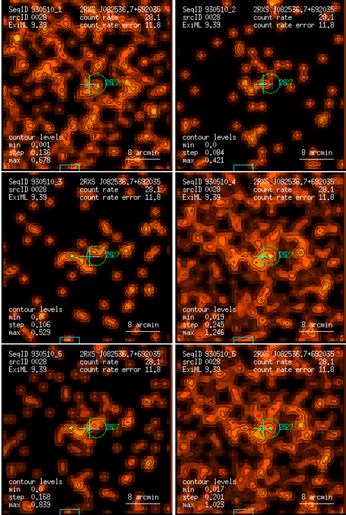
Figure 28: RASS 930510: detection 0028: band rate images, Gaussian filter: (1) PSPC channels 11 – 41, (2) 52 – 90, (3) 91 – 201, (4) 11 – 235, (5) 52 – 201, (6) 11 – 201. Broad band rates in counts/ks. Band rate contour levels in counts/ks/arcmin 2 .
