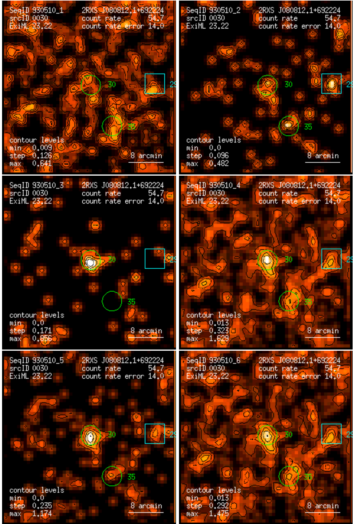
Figure 30: RASS 930510: detection 0030: band rate images, Gaussian filter: (1) PSPC channels 11 – 41, (2) 52 – 90, (3) 91 – 201, (4) 11 – 235, (5) 52 – 201, (6) 11 – 201. Broad band rates in counts/ks. Band rate contour levels in counts/ks/arcmin 2 .
