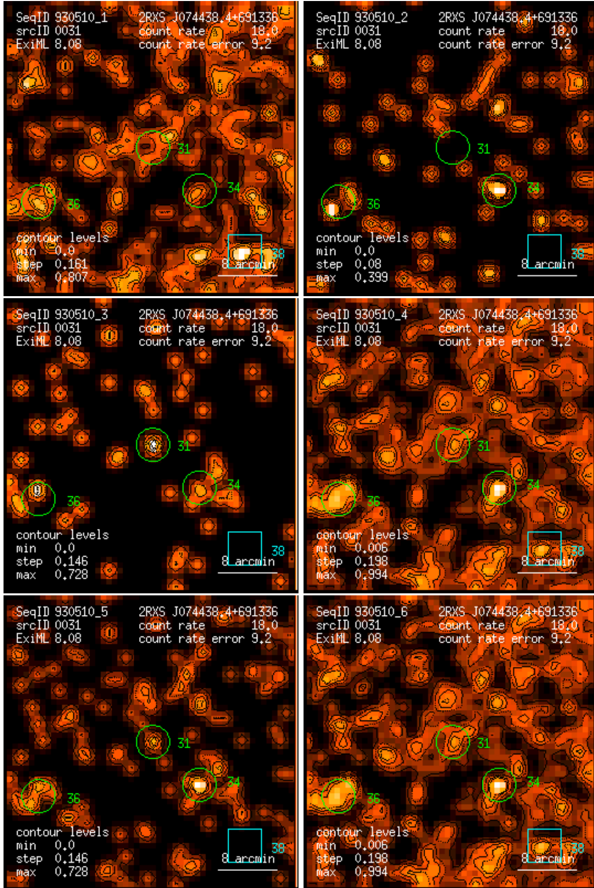
Figure 31: RASS 930510: detection 0031: band rate images, Gaussian filter: (1) PSPC channels 11 – 41, (2) 52 – 90, (3) 91 – 201, (4) 11 – 235, (5) 52 – 201, (6) 11 – 201. Broad band rates in counts/ks. Band rate contour levels in counts/ks/arcmin 2 .
