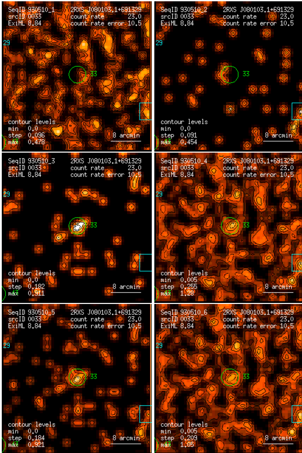
Figure 33: RASS 930510: detection 0033: band rate images, Gaussian filter: (1) PSPC channels 11 – 41, (2) 52 – 90, (3) 91 – 201, (4) 11 – 235, (5) 52 – 201, (6) 11 – 201. Broad band rates in counts/ks. Band rate contour levels in counts/ks/arcmin 2 .
