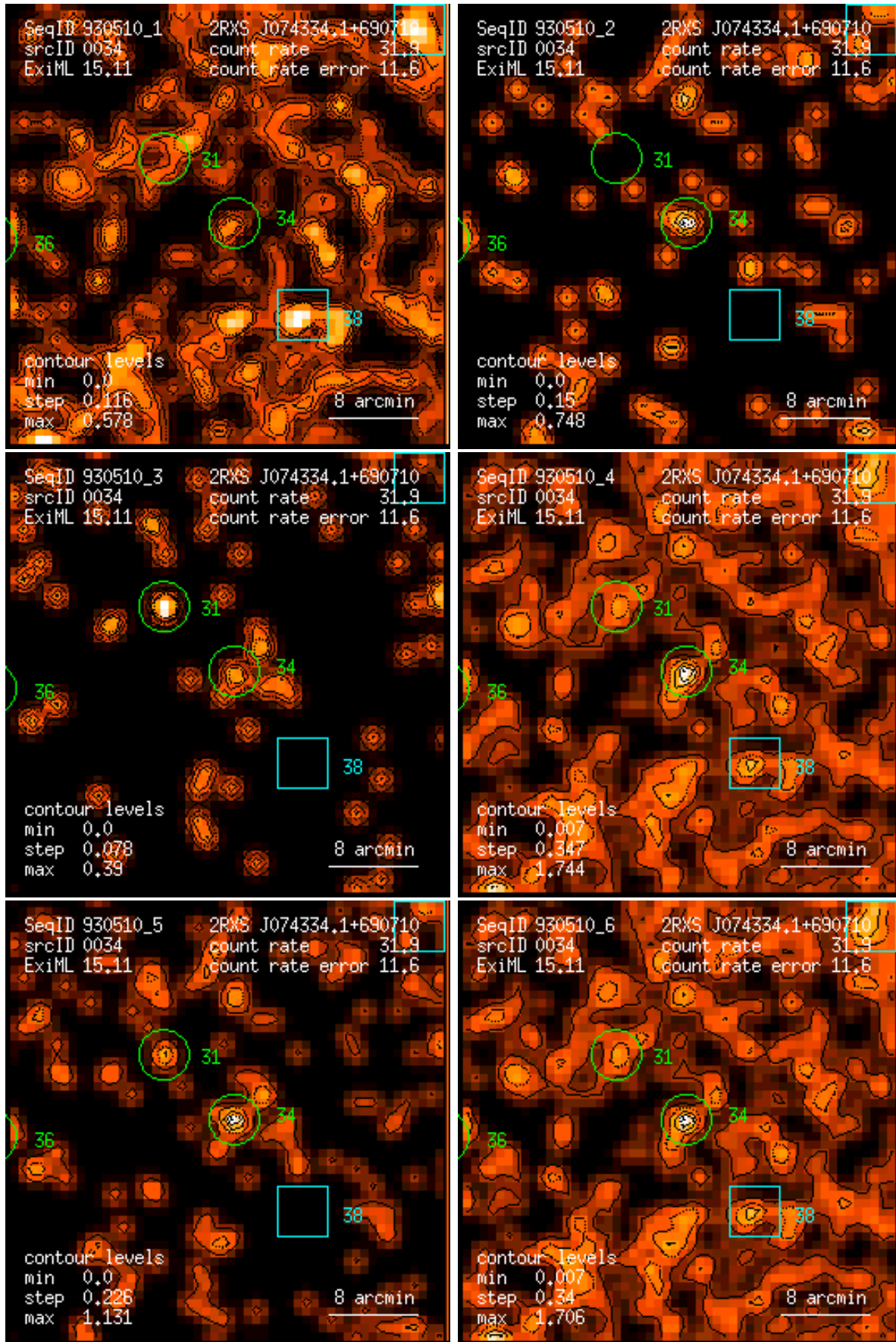
Figure 34: RASS 930510: detection 0034: band rate images, Gaussian filter: (1) PSPC channels 11 – 41, (2) 52 – 90, (3) 91 – 201, (4) 11 – 235, (5) 52 – 201, (6) 11 – 201. Broad band rates in counts/ks. Band rate contour levels in counts/ks/arcmin 2 .
