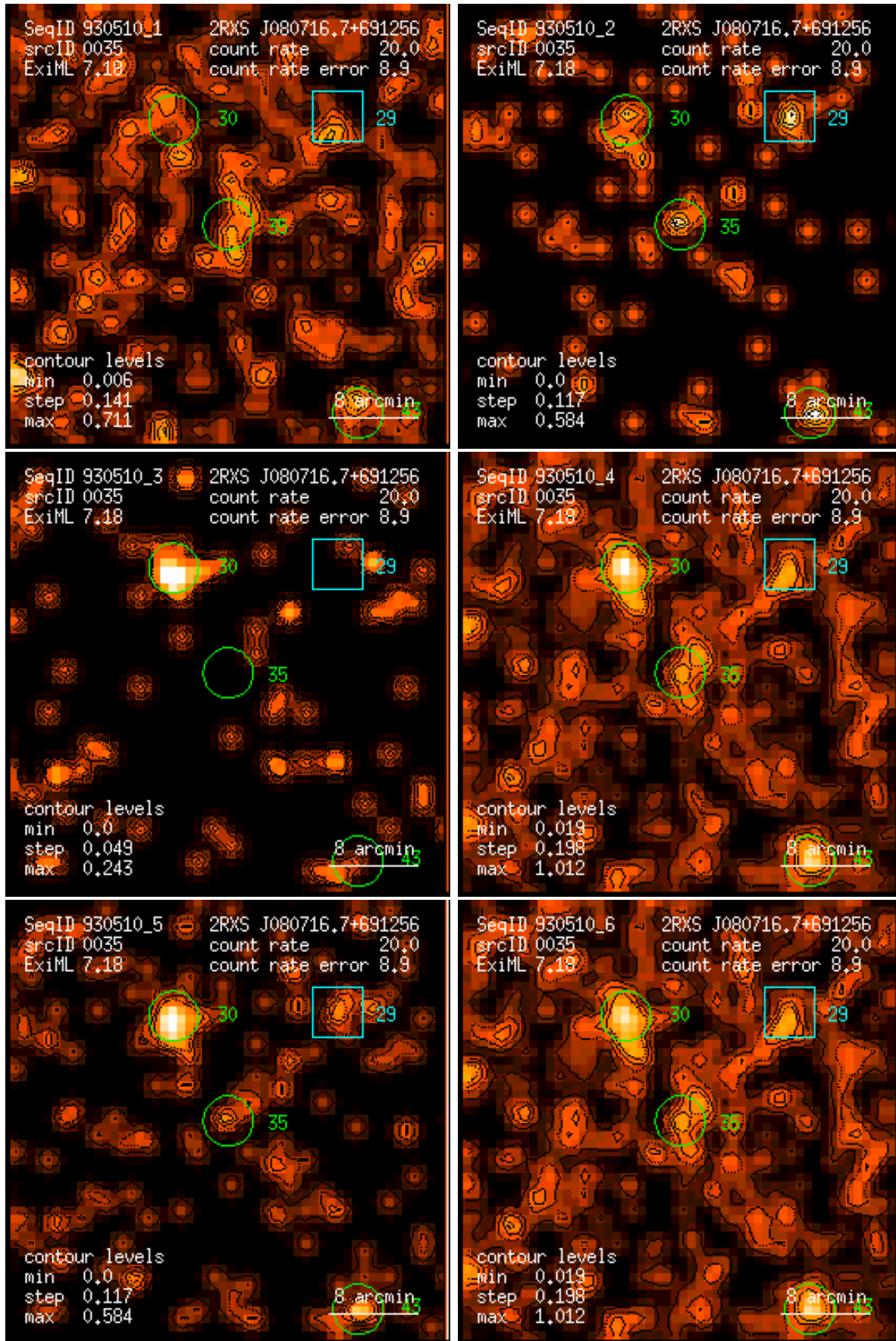
Figure 35: RASS 930510: detection 0035: band rate images, Gaussian filter: (1) PSPC channels 11 – 41, (2) 52 – 90, (3) 91 – 201, (4) 11 – 235, (5) 52 – 201, (6) 11 – 201. Broad band rates in counts/ks. Band rate contour levels in counts/ks/arcmin 2 .
