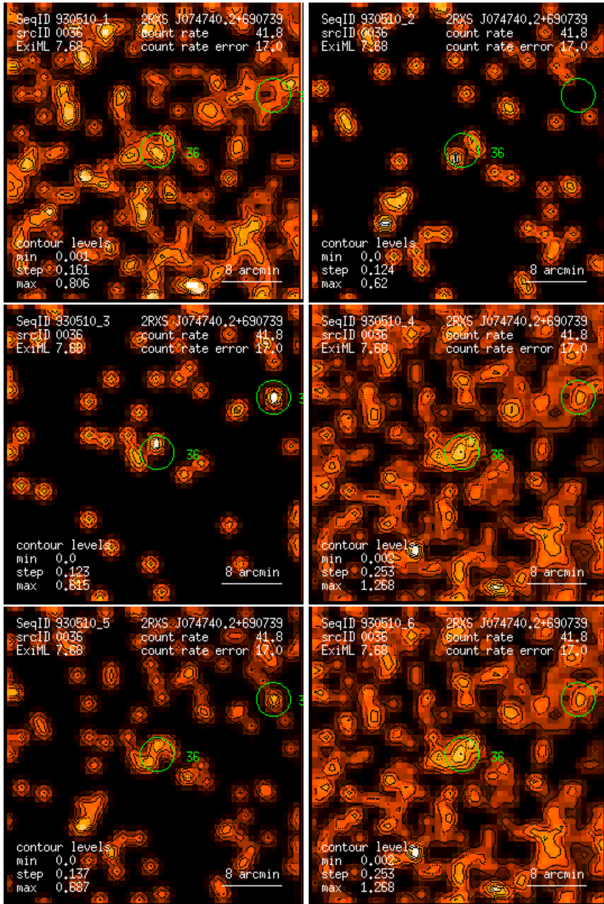
Figure 36: RASS 930510: detection 0036: band rate images, Gaussian filter: (1) PSPC channels 11 – 41, (2) 52 – 90, (3) 91 – 201, (4) 11 – 235, (5) 52 – 201, (6) 11 – 201. Broad band rates in counts/ks. Band rate contour levels in counts/ks/arcmin 2 .
