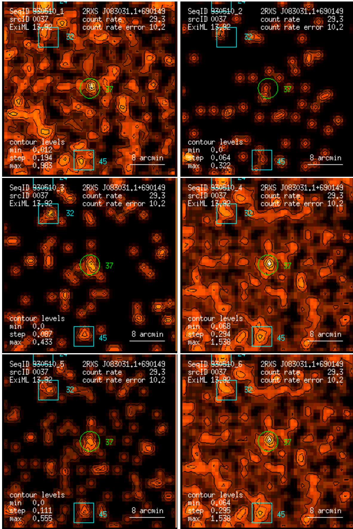
Figure 37: RASS 930510: detection 0037: band rate images, Gaussian filter: (1) PSPC channels 11 – 41, (2) 52 – 90, (3) 91 – 201, (4) 11 – 235, (5) 52 – 201, (6) 11 – 201. Broad band rates in counts/ks. Band rate contour levels in counts/ks/arcmin 2 .
