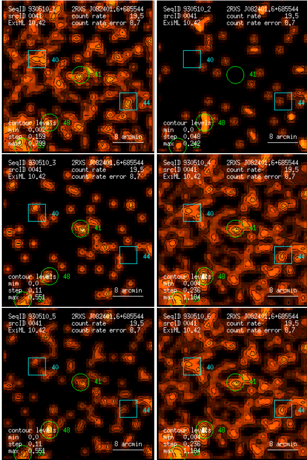
Figure 41: RASS 930510: detection 0041: band rate images, Gaussian filter: (1) PSPC channels 11 – 41, (2) 52 – 90, (3) 91 – 201, (4) 11 – 235, (5) 52 – 201, (6) 11 – 201. Broad band rates in counts/ks. Band rate contour levels in counts/ks/arcmin 2 .
