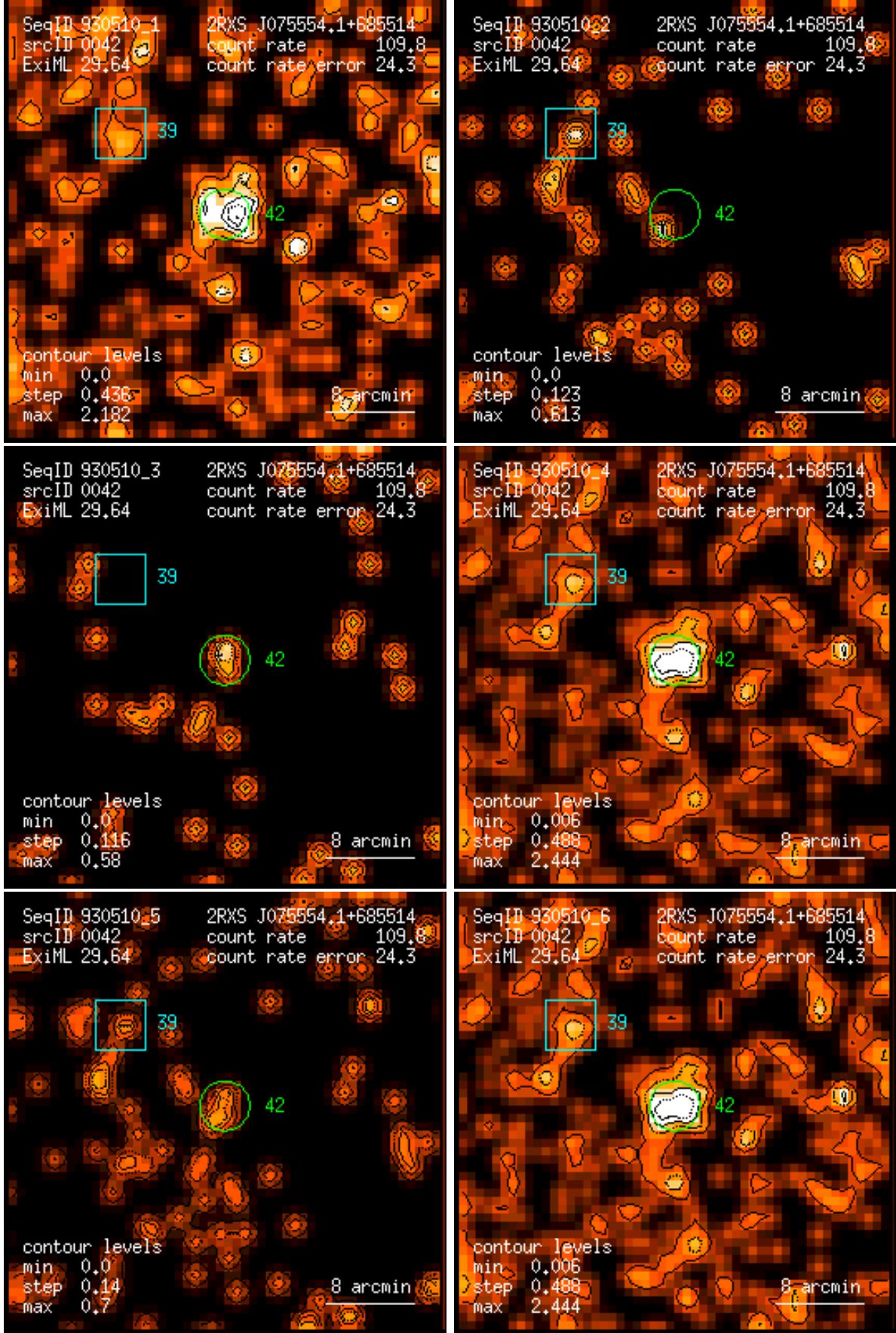
Figure 42: RASS 930510: detection 0042: band rate images, Gaussian filter: (1) PSPC channels 11 – 41, (2) 52 – 90, (3) 91 – 201, (4) 11 – 235, (5) 52 – 201, (6) 11 – 201. Broad band rates in counts/ks. Band rate contour levels in counts/ks/arcmin 2 .
