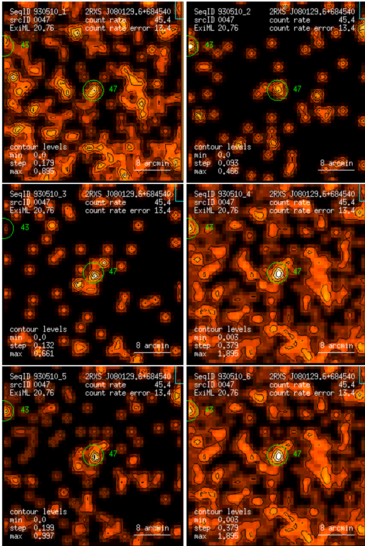
Figure 47: RASS 930510: detection 0047: band rate images, Gaussian filter: (1) PSPC channels 11 – 41, (2) 52 – 90, (3) 91 – 201, (4) 11 – 235, (5) 52 – 201, (6) 11 – 201. Broad band rates in counts/ks. Band rate contour levels in counts/ks/arcmin 2 .
