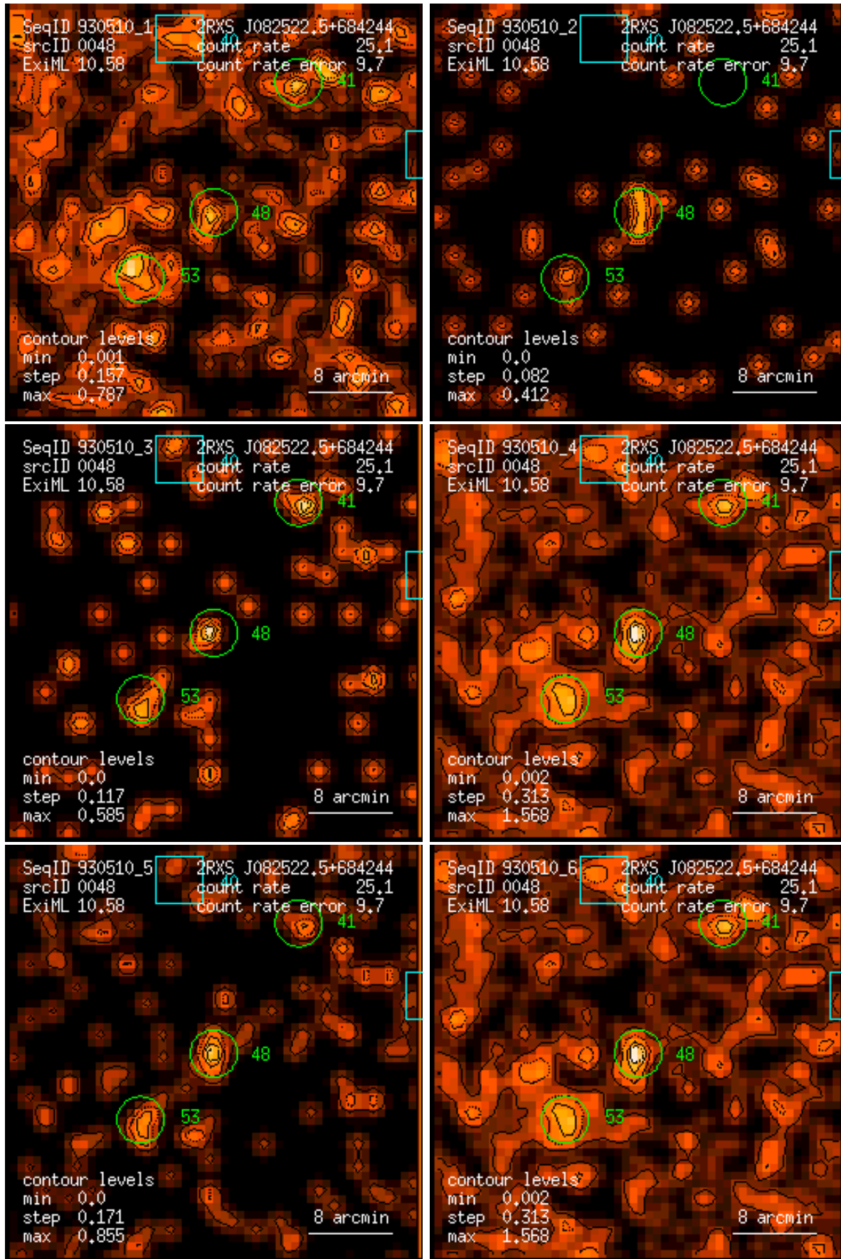
Figure 48: RASS 930510: detection 0048: band rate images, Gaussian filter: (1) PSPC channels 11 – 41, (2) 52 – 90, (3) 91 – 201, (4) 11 – 235, (5) 52 – 201, (6) 11 – 201. Broad band rates in counts/ks. Band rate contour levels in counts/ks/arcmin 2 .
