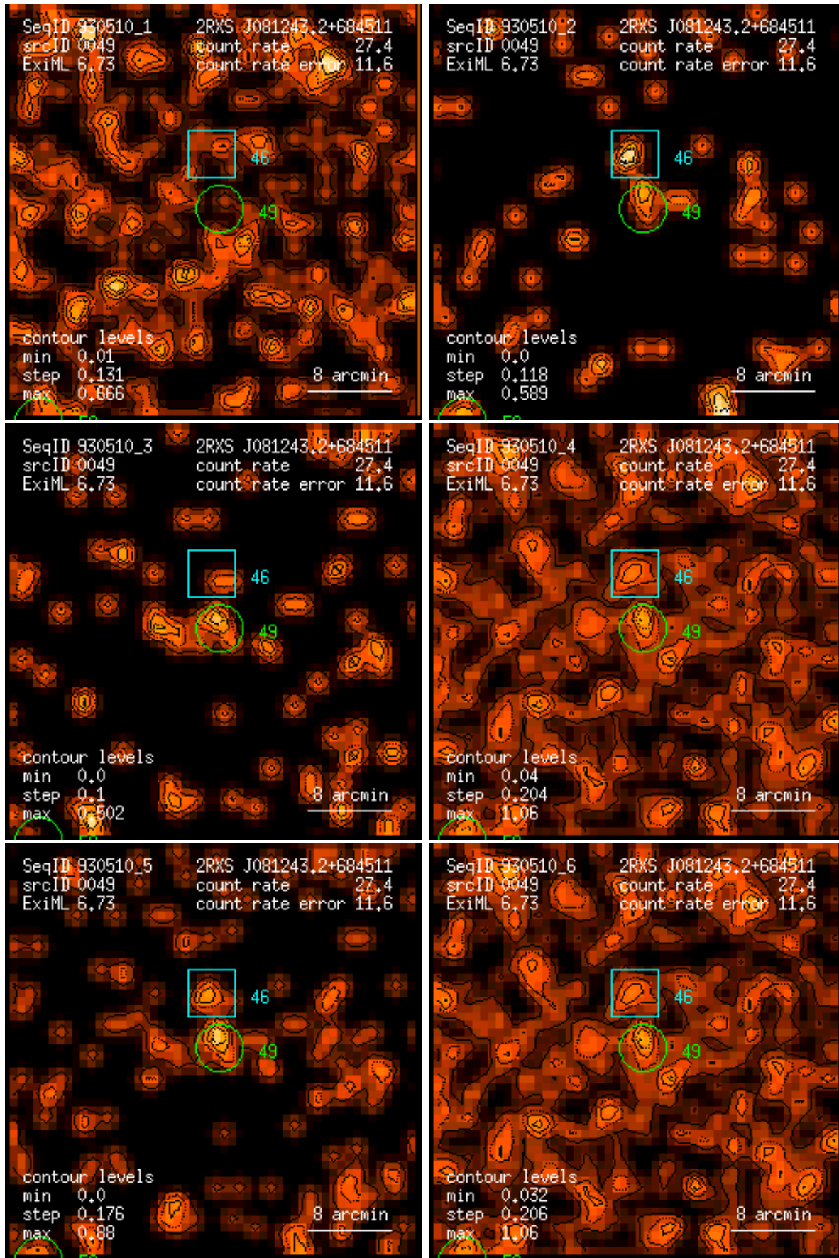
Figure 49: RASS 930510: detection 0049: band rate images, Gaussian filter: (1) PSPC channels 11 – 41, (2) 52 – 90, (3) 91 – 201, (4) 11 – 235, (5) 52 – 201, (6) 11 – 201. Broad band rates in counts/ks. Band rate contour levels in counts/ks/arcmin 2 .
