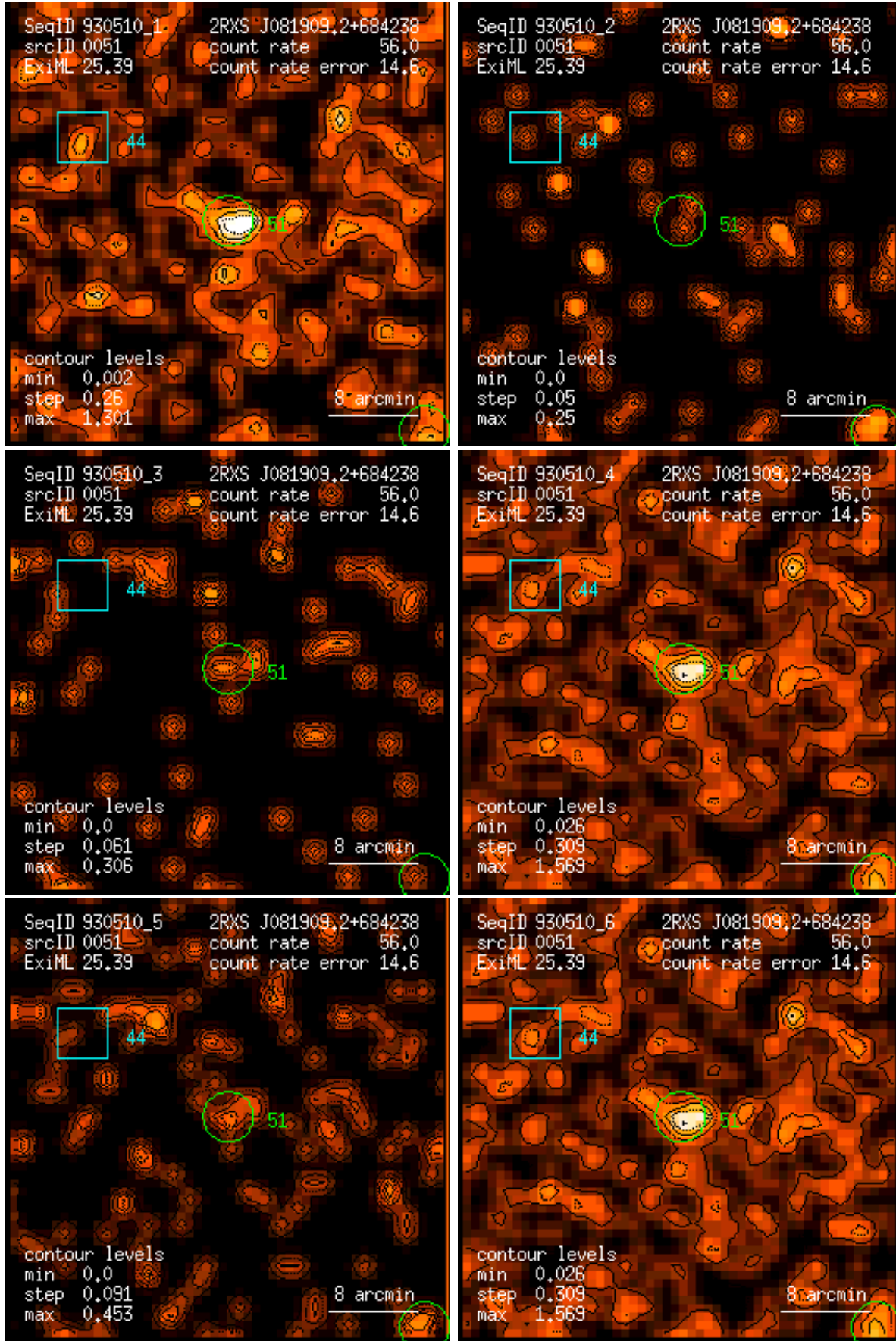
Figure 51: RASS 930510: detection 0051: band rate images, Gaussian filter: (1) PSPC channels 11 – 41, (2) 52 – 90, (3) 91 – 201, (4) 11 – 235, (5) 52 – 201, (6) 11 – 201. Broad band rates in counts/ks. Band rate contour levels in counts/ks/arcmin 2 .
