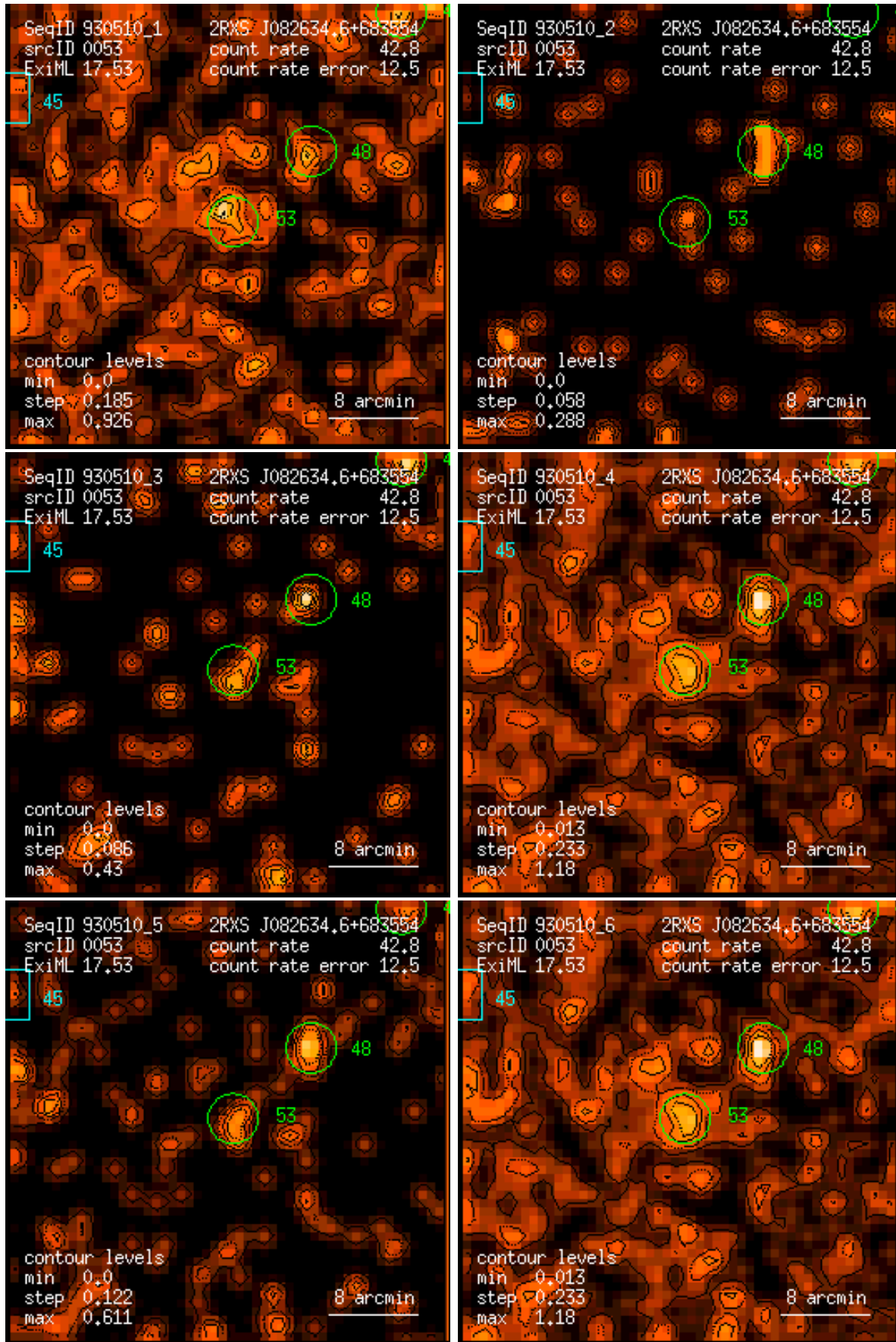
Figure 53: RASS 930510: detection 0053: band rate images, Gaussian filter: (1) PSPC channels 11 – 41, (2) 52 – 90, (3) 91 – 201, (4) 11 – 235, (5) 52 – 201, (6) 11 – 201. Broad band rates in counts/ks. Band rate contour levels in counts/ks/arcmin 2 .
