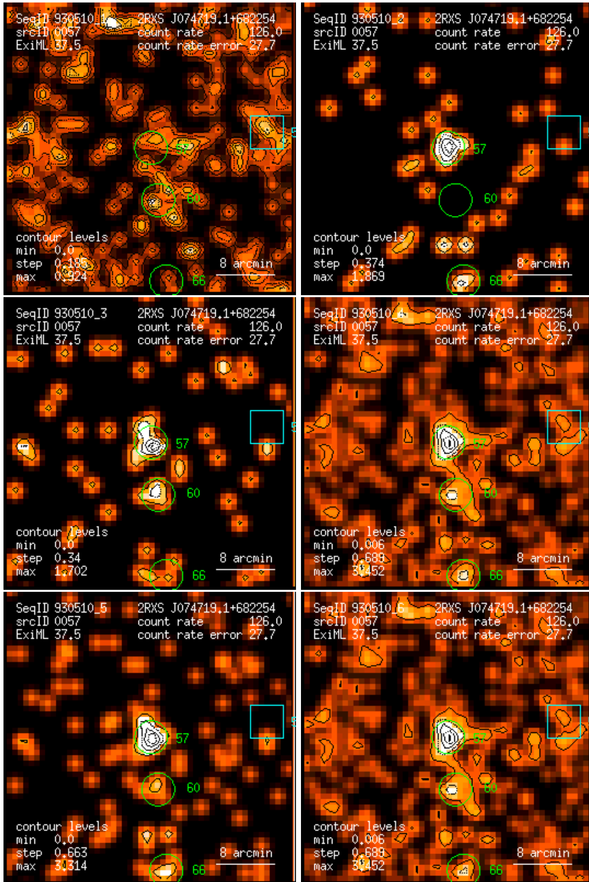
Figure 57: RASS 930510: detection 0057: band rate images, Gaussian filter: (1) PSPC channels 11 – 41, (2) 52 – 90, (3) 91 – 201, (4) 11 – 235, (5) 52 – 201, (6) 11 – 201. Broad band rates in counts/ks. Band rate contour levels in counts/ks/arcmin 2 .
