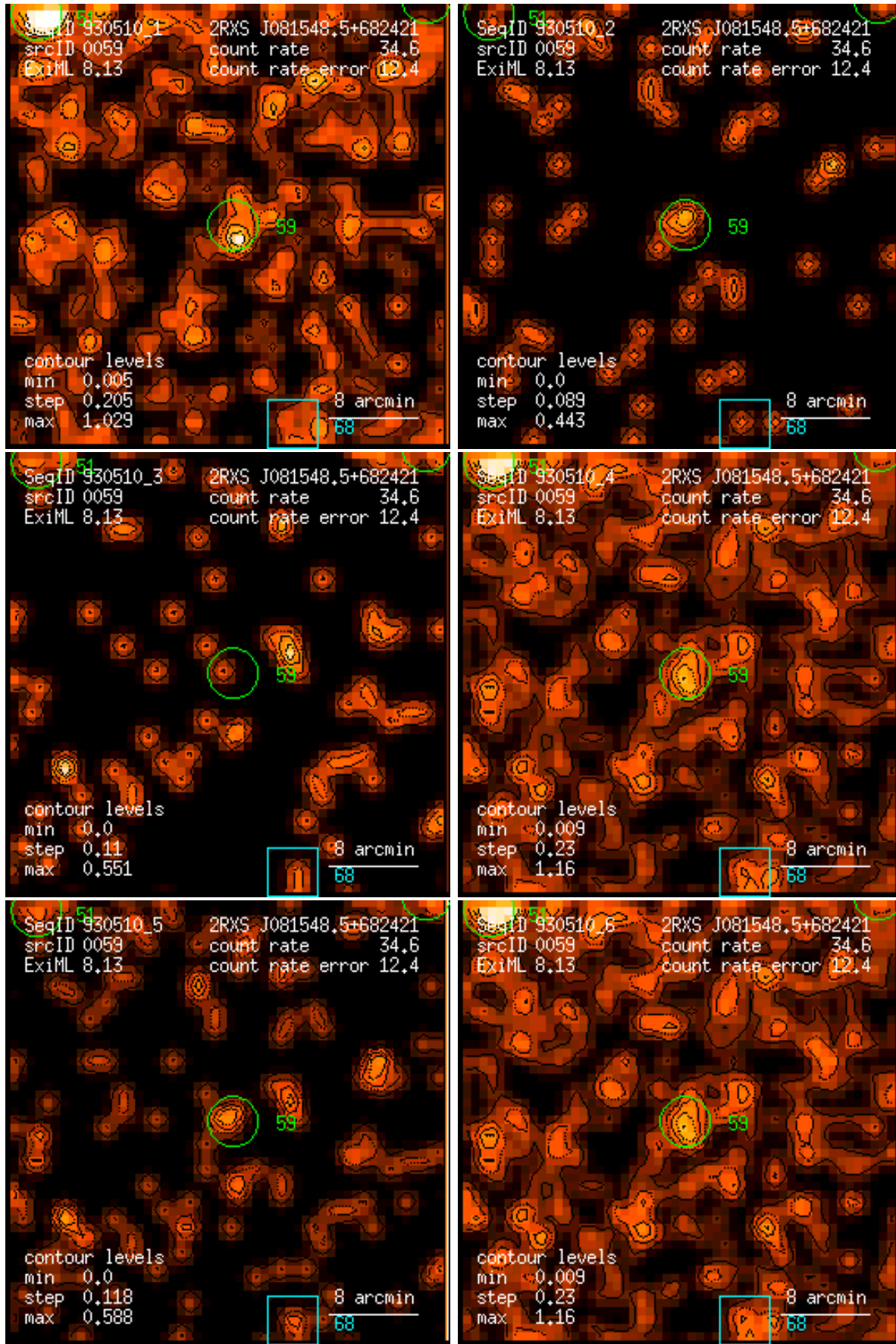
Figure 59: RASS 930510: detection 0059: band rate images, Gaussian filter: (1) PSPC channels 11 – 41, (2) 52 – 90, (3) 91 – 201, (4) 11 – 235, (5) 52 – 201, (6) 11 – 201. Broad band rates in counts/ks. Band rate contour levels in counts/ks/arcmin 2 .
