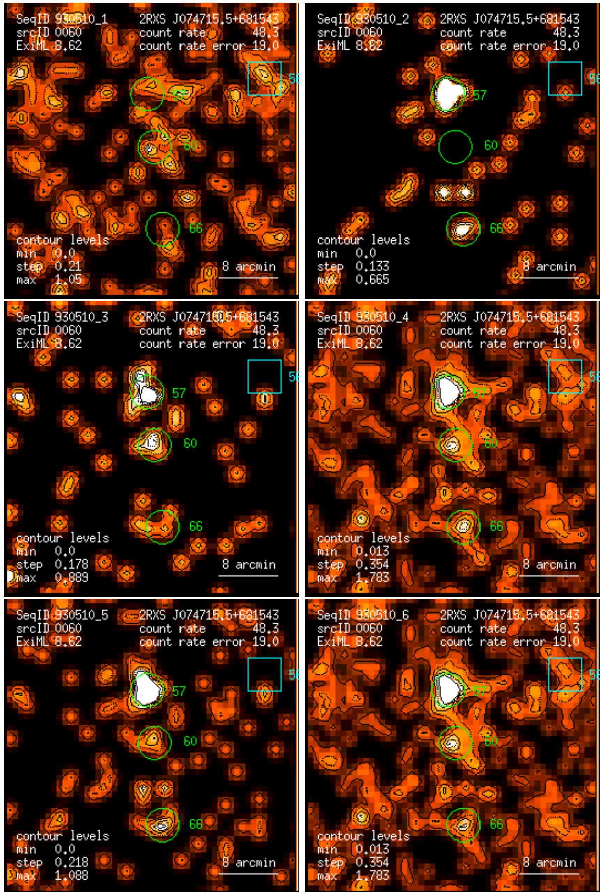
Figure 60: RASS 930510: detection 0060: band rate images, Gaussian filter: (1) PSPC channels 11 – 41, (2) 52 – 90, (3) 91 – 201, (4) 11 – 235, (5) 52 – 201, (6) 11 – 201. Broad band rates in counts/ks. Band rate contour levels in counts/ks/arcmin 2 .
