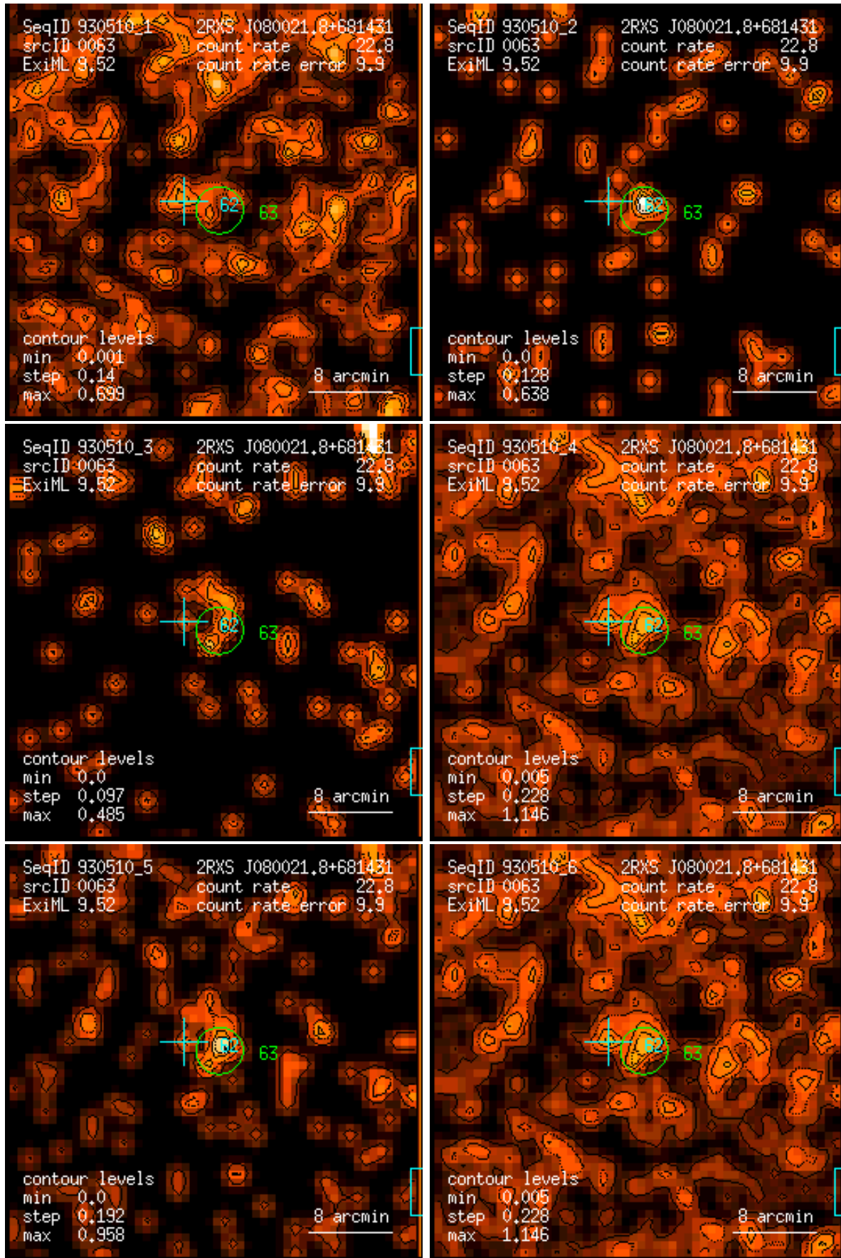
Figure 63: RASS 930510: detection 0063: band rate images, Gaussian filter: (1) PSPC channels 11 – 41, (2) 52 – 90, (3) 91 – 201, (4) 11 – 235, (5) 52 – 201, (6) 11 – 201. Broad band rates in counts/ks. Band rate contour levels in counts/ks/arcmin 2 .
