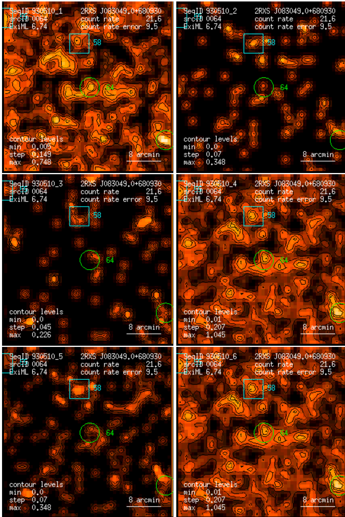
Figure 64: RASS 930510: detection 0064: band rate images, Gaussian filter: (1) PSPC channels 11 – 41, (2) 52 – 90, (3) 91 – 201, (4) 11 – 235, (5) 52 – 201, (6) 11 – 201. Broad band rates in counts/ks. Band rate contour levels in counts/ks/arcmin 2 .
