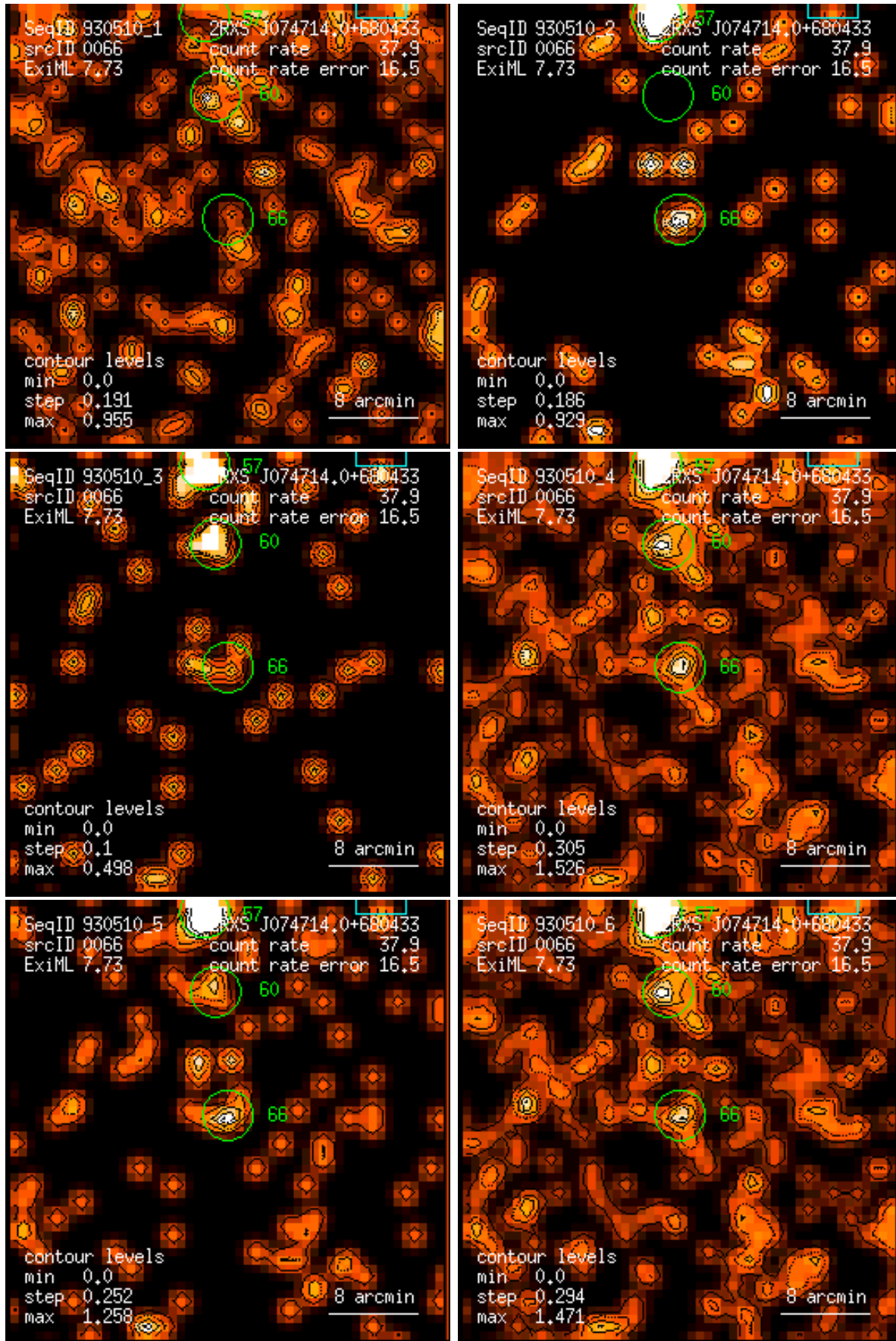
Figure 66: RASS 930510: detection 0066: band rate images, Gaussian filter: (1) PSPC channels 11 – 41, (2) 52 – 90, (3) 91 – 201, (4) 11 – 235, (5) 52 – 201, (6) 11 – 201. Broad band rates in counts/ks. Band rate contour levels in counts/ks/arcmin 2 .
