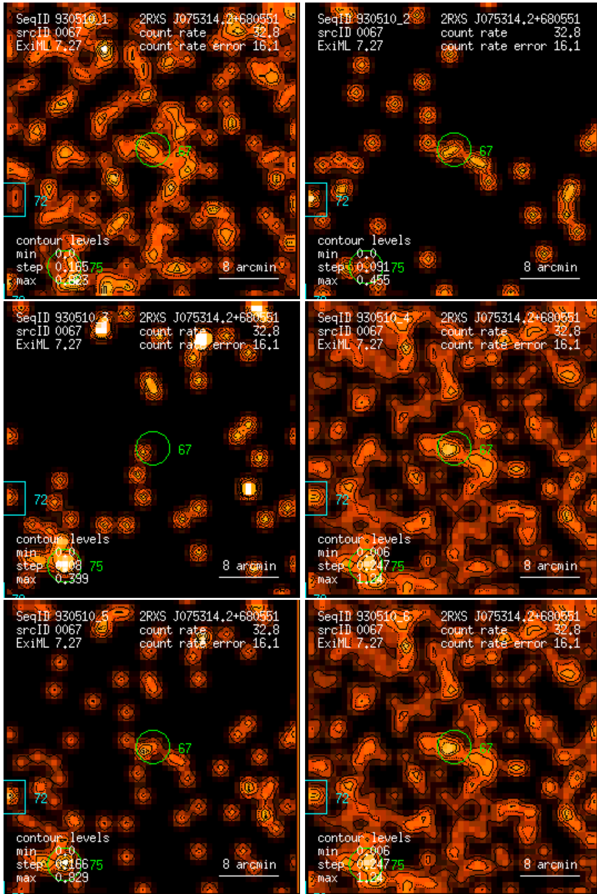
Figure 67: RASS 930510: detection 0067: band rate images, Gaussian filter: (1) PSPC channels 11 – 41, (2) 52 – 90, (3) 91 – 201, (4) 11 – 235, (5) 52 – 201, (6) 11 – 201. Broad band rates in counts/ks. Band rate contour levels in counts/ks/arcmin 2 .
