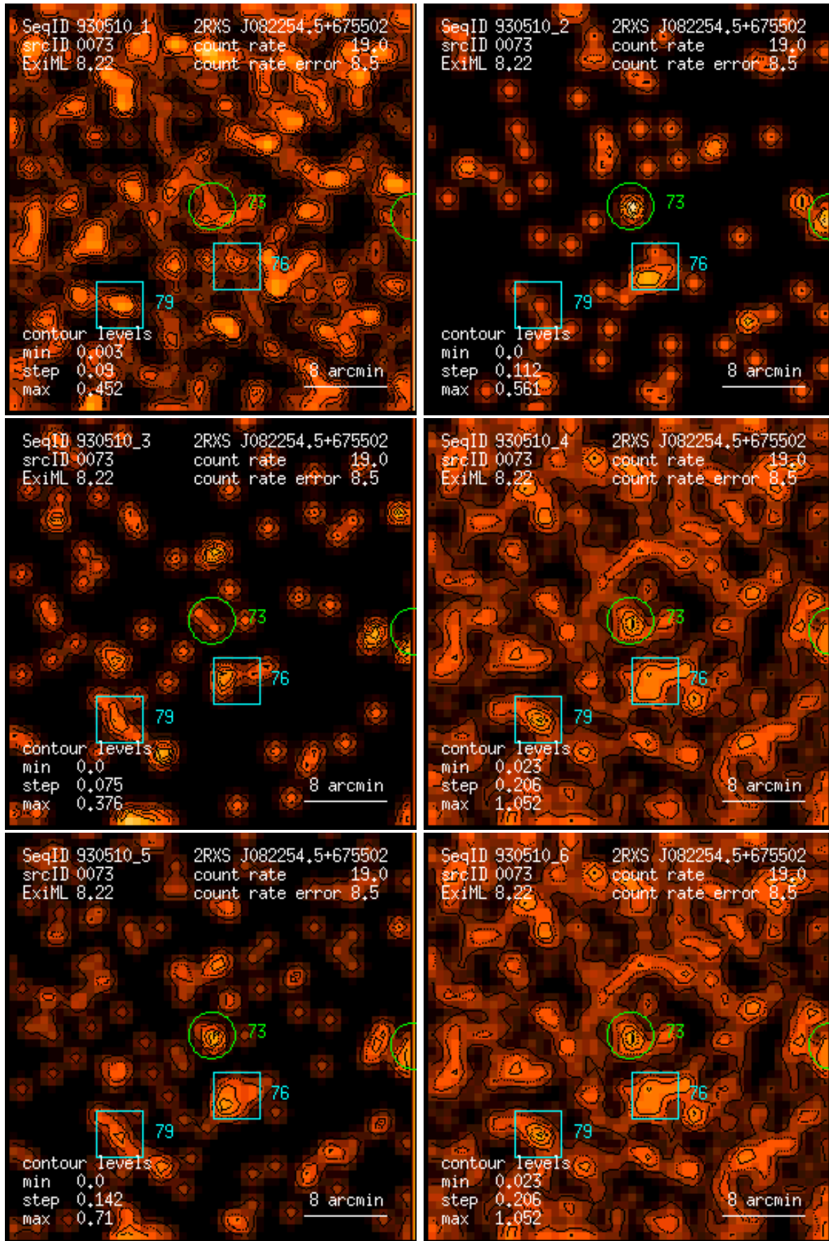
Figure 73: RASS 930510: detection 0073: band rate images, Gaussian filter: (1) PSPC channels 11 – 41, (2) 52 – 90, (3) 91 – 201, (4) 11 – 235, (5) 52 – 201, (6) 11 – 201. Broad band rates in counts/ks. Band rate contour levels in counts/ks/arcmin 2 .
