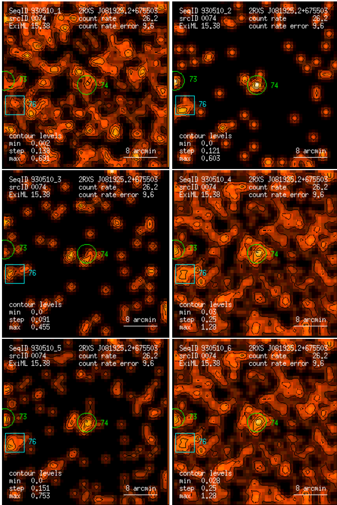
Figure 74: RASS 930510: detection 0074: band rate images, Gaussian filter: (1) PSPC channels 11 – 41, (2) 52 – 90, (3) 91 – 201, (4) 11 – 235, (5) 52 – 201, (6) 11 – 201. Broad band rates in counts/ks. Band rate contour levels in counts/ks/arcmin 2 .
