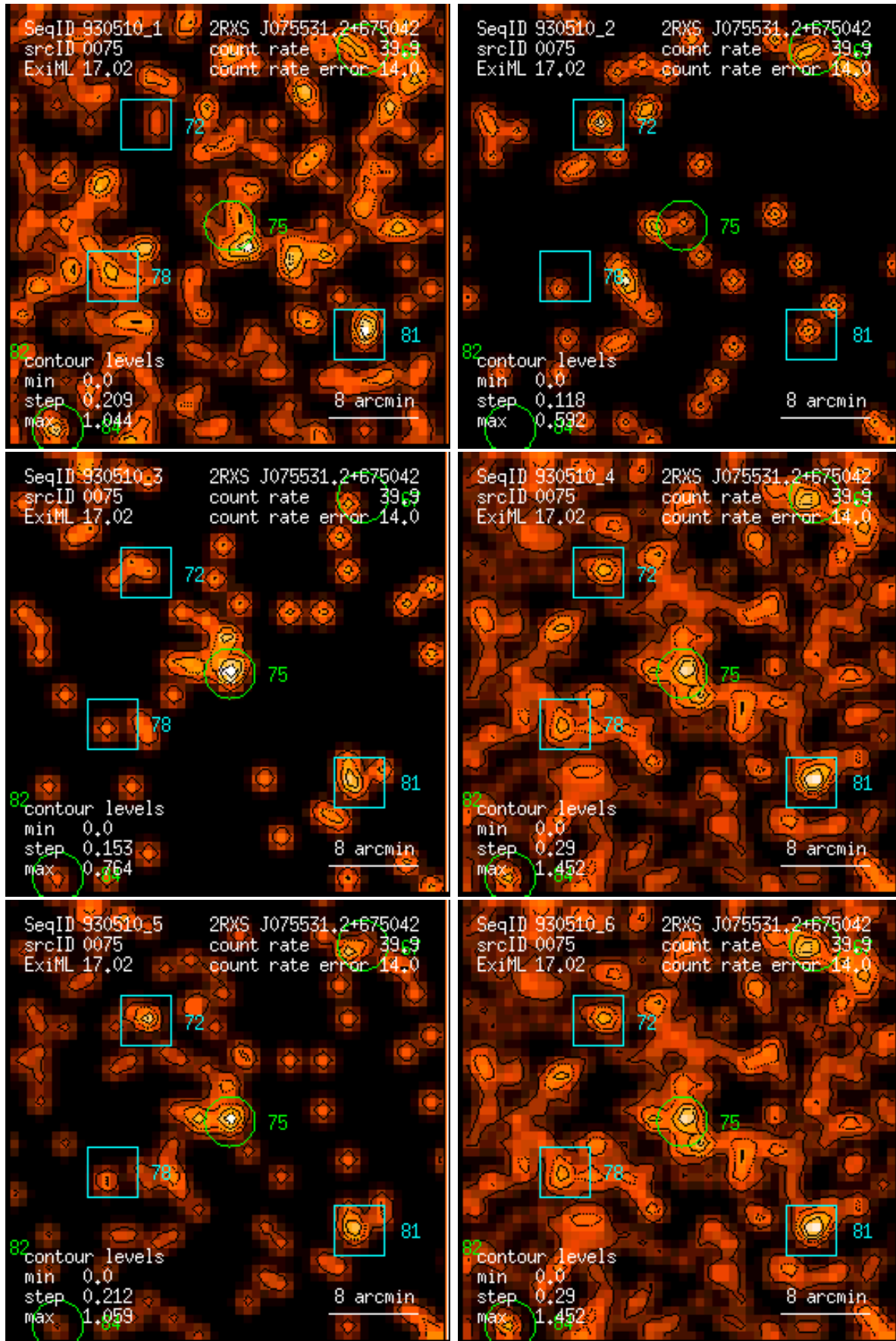
Figure 75: RASS 930510: detection 0075: band rate images, Gaussian filter: (1) PSPC channels 11 – 41, (2) 52 – 90, (3) 91 – 201, (4) 11 – 235, (5) 52 – 201, (6) 11 – 201. Broad band rates in counts/ks. Band rate contour levels in counts/ks/arcmin 2 .
