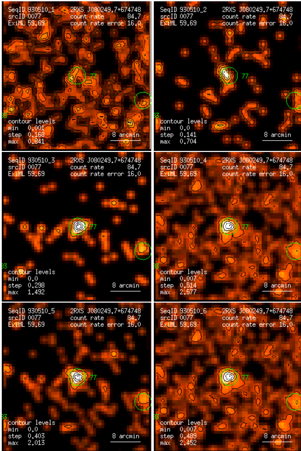
Figure 77: RASS 930510: detection 0077: band rate images, Gaussian filter: (1) PSPC channels 11 – 41, (2) 52 – 90, (3) 91 – 201, (4) 11 – 235, (5) 52 – 201, (6) 11 – 201. Broad band rates in counts/ks. Band rate contour levels in counts/ks/arcmin 2 .
