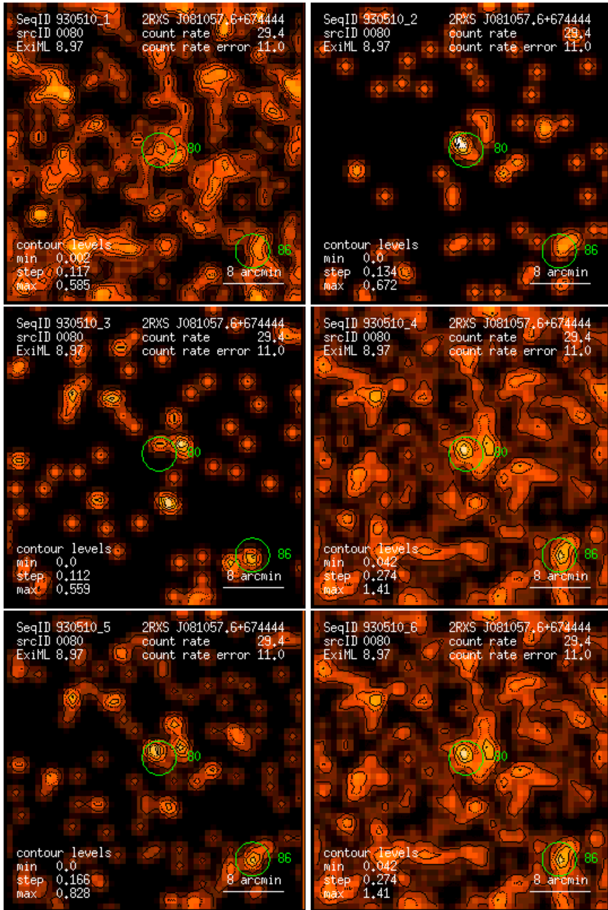
Figure 80: RASS 930510: detection 0080: band rate images, Gaussian filter: (1) PSPC channels 11 – 41, (2) 52 – 90, (3) 91 – 201, (4) 11 – 235, (5) 52 – 201, (6) 11 – 201. Broad band rates in counts/ks. Band rate contour levels in counts/ks/arcmin 2 .
