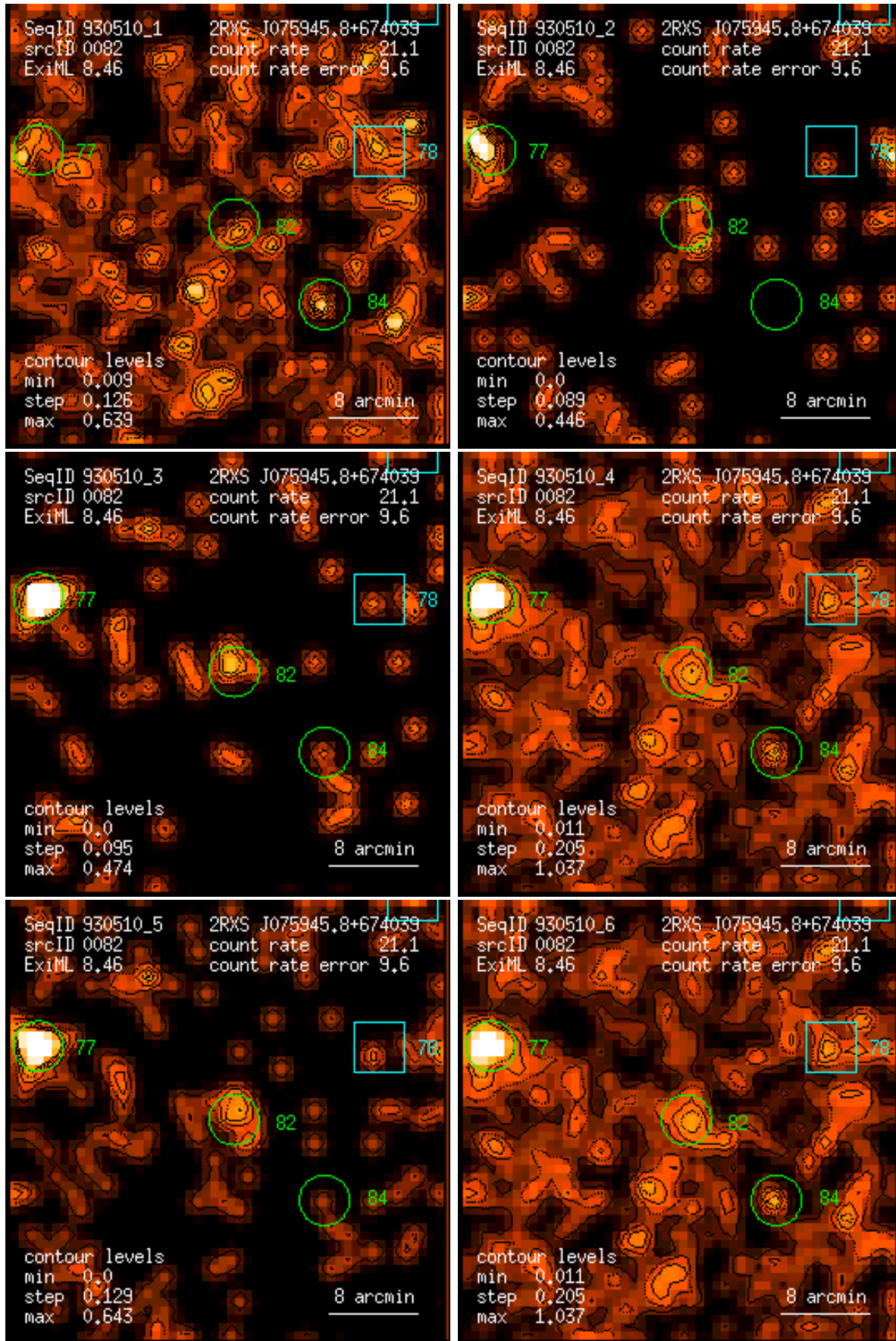
Figure 82: RASS 930510: detection 0082: band rate images, Gaussian filter: (1) PSPC channels 11 – 41, (2) 52 – 90, (3) 91 – 201, (4) 11 – 235, (5) 52 – 201, (6) 11 – 201. Broad band rates in counts/ks. Band rate contour levels in counts/ks/arcmin 2 .
