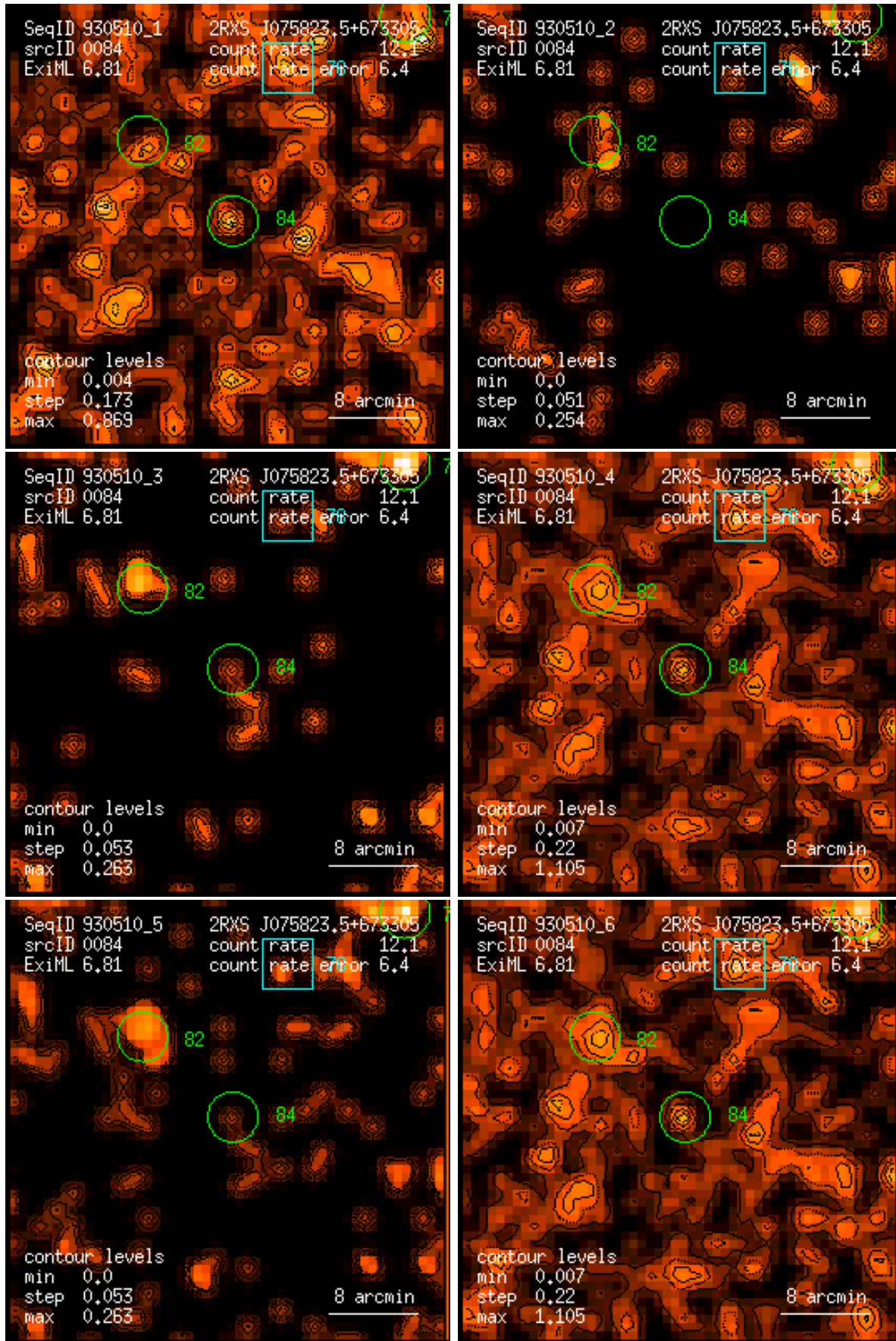
Figure 84: RASS 930510: detection 0084: band rate images, Gaussian filter: (1) PSPC channels 11 – 41, (2) 52 – 90, (3) 91 – 201, (4) 11 – 235, (5) 52 – 201, (6) 11 – 201. Broad band rates in counts/ks. Band rate contour levels in counts/ks/arcmin 2 .
