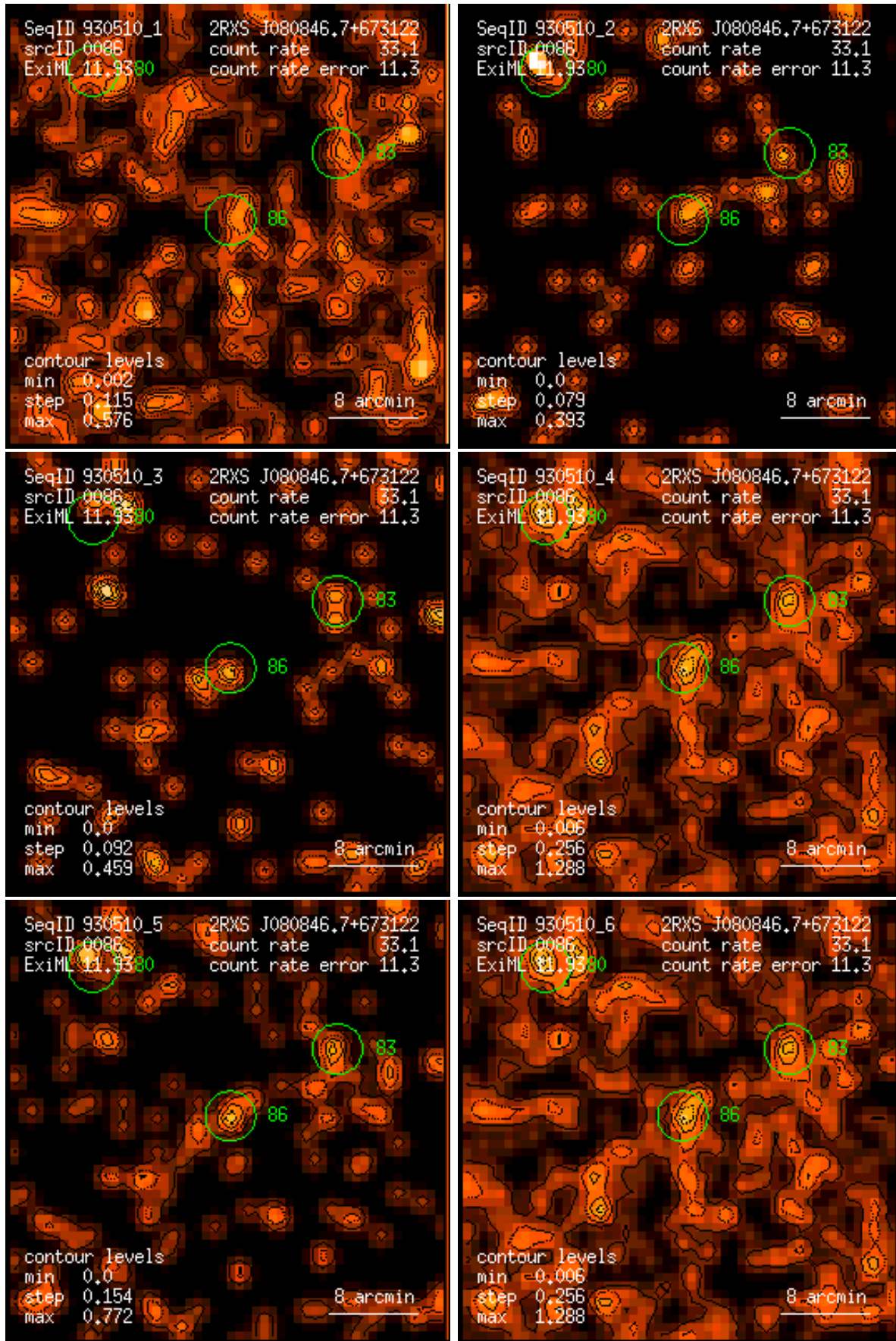
Figure 86: RASS 930510: detection 0086: band rate images, Gaussian filter: (1) PSPC channels 11 – 41, (2) 52 – 90, (3) 91 – 201, (4) 11 – 235, (5) 52 – 201, (6) 11 – 201. Broad band rates in counts/ks. Band rate contour levels in counts/ks/arcmin 2 .
