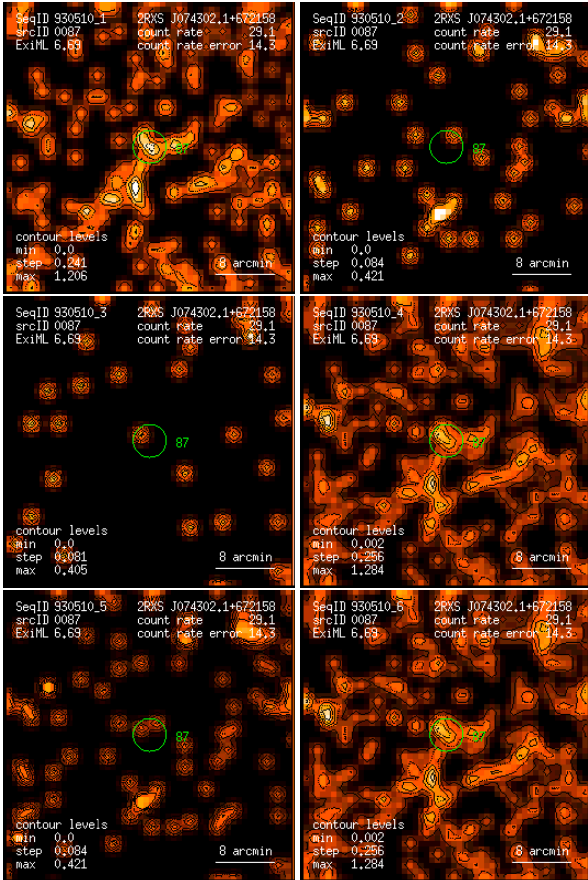
Figure 87: RASS 930510: detection 0087: band rate images, Gaussian filter: (1) PSPC channels 11 – 41, (2) 52 – 90, (3) 91 – 201, (4) 11 – 235, (5) 52 – 201, (6) 11 – 201. Broad band rates in counts/ks. Band rate contour levels in counts/ks/arcmin 2 .
