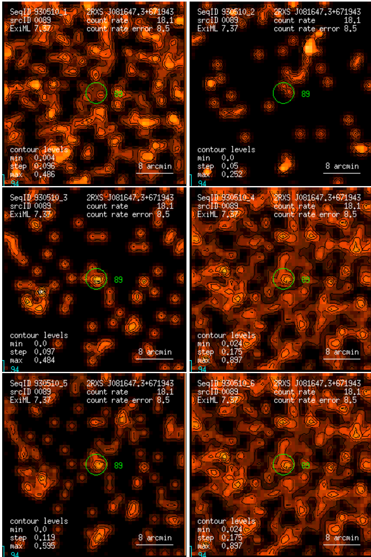
Figure 89: RASS 930510: detection 0089: band rate images, Gaussian filter: (1) PSPC channels 11 – 41, (2) 52 – 90, (3) 91 – 201, (4) 11 – 235, (5) 52 – 201, (6) 11 – 201. Broad band rates in counts/ks. Band rate contour levels in counts/ks/arcmin 2 .
