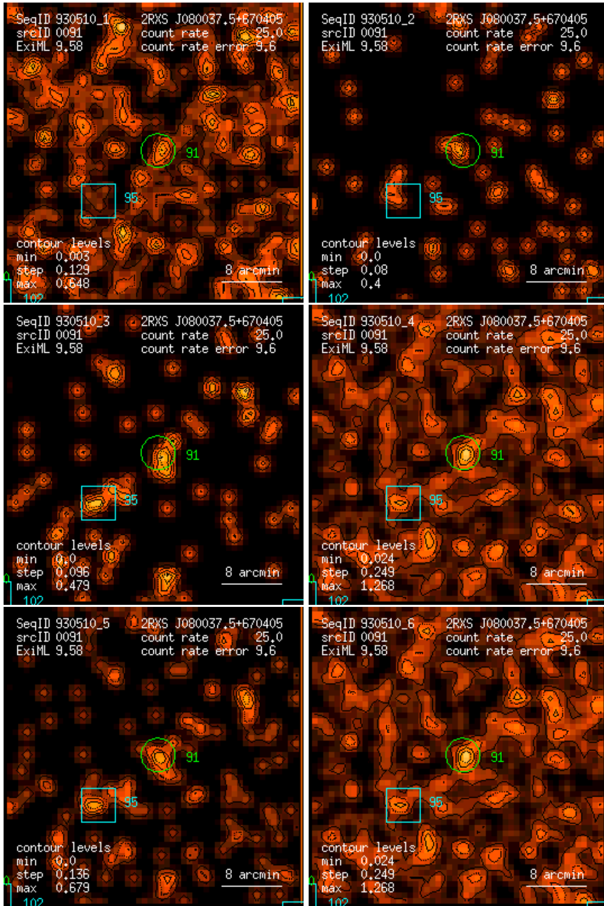
Figure 91: RASS 930510: detection 0091: band rate images, Gaussian filter: (1) PSPC channels 11 – 41, (2) 52 – 90, (3) 91 – 201, (4) 11 – 235, (5) 52 – 201, (6) 11 – 201. Broad band rates in counts/ks. Band rate contour levels in counts/ks/arcmin 2 .
