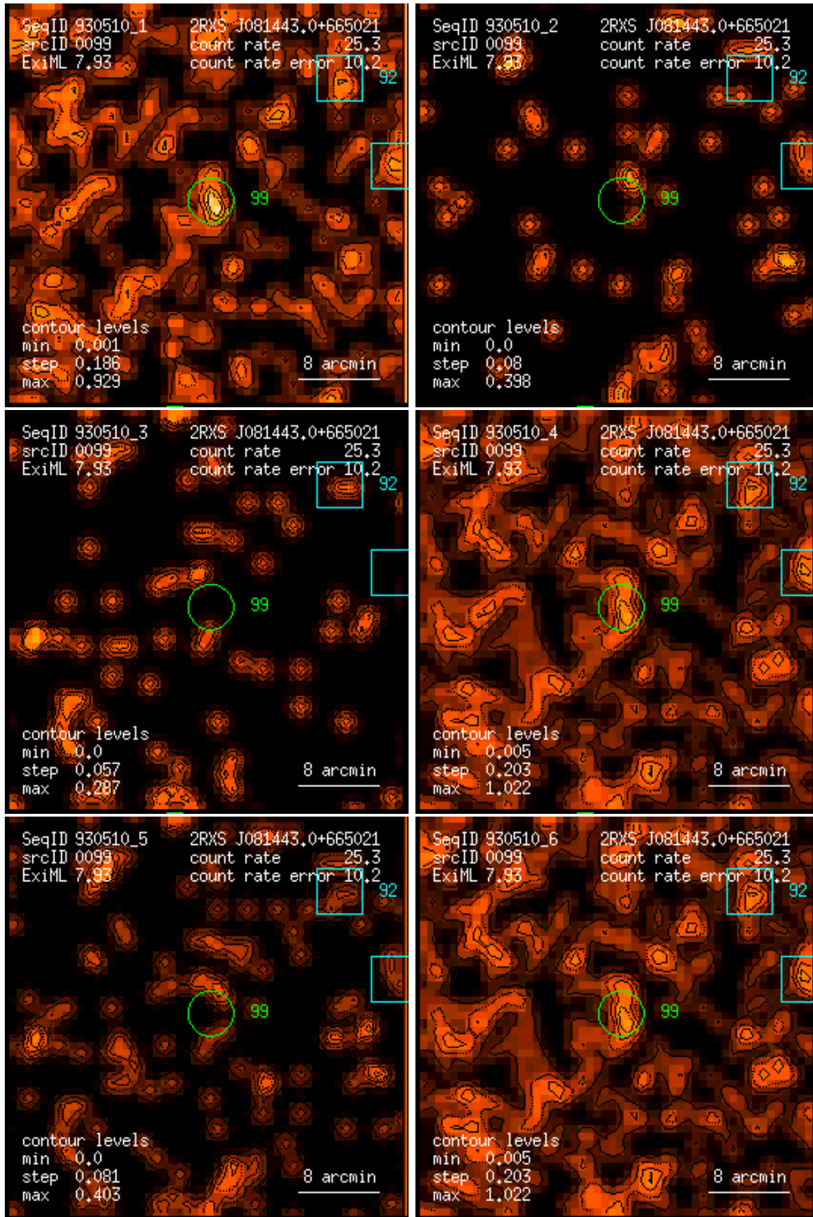
Figure 99: RASS 930510: detection 0099: band rate images, Gaussian filter: (1) PSPC channels 11 – 41, (2) 52 – 90, (3) 91 – 201, (4) 11 – 235, (5) 52 – 201, (6) 11 – 201. Broad band rates in counts/ks. Band rate contour levels in counts/ks/arcmin 2 .
