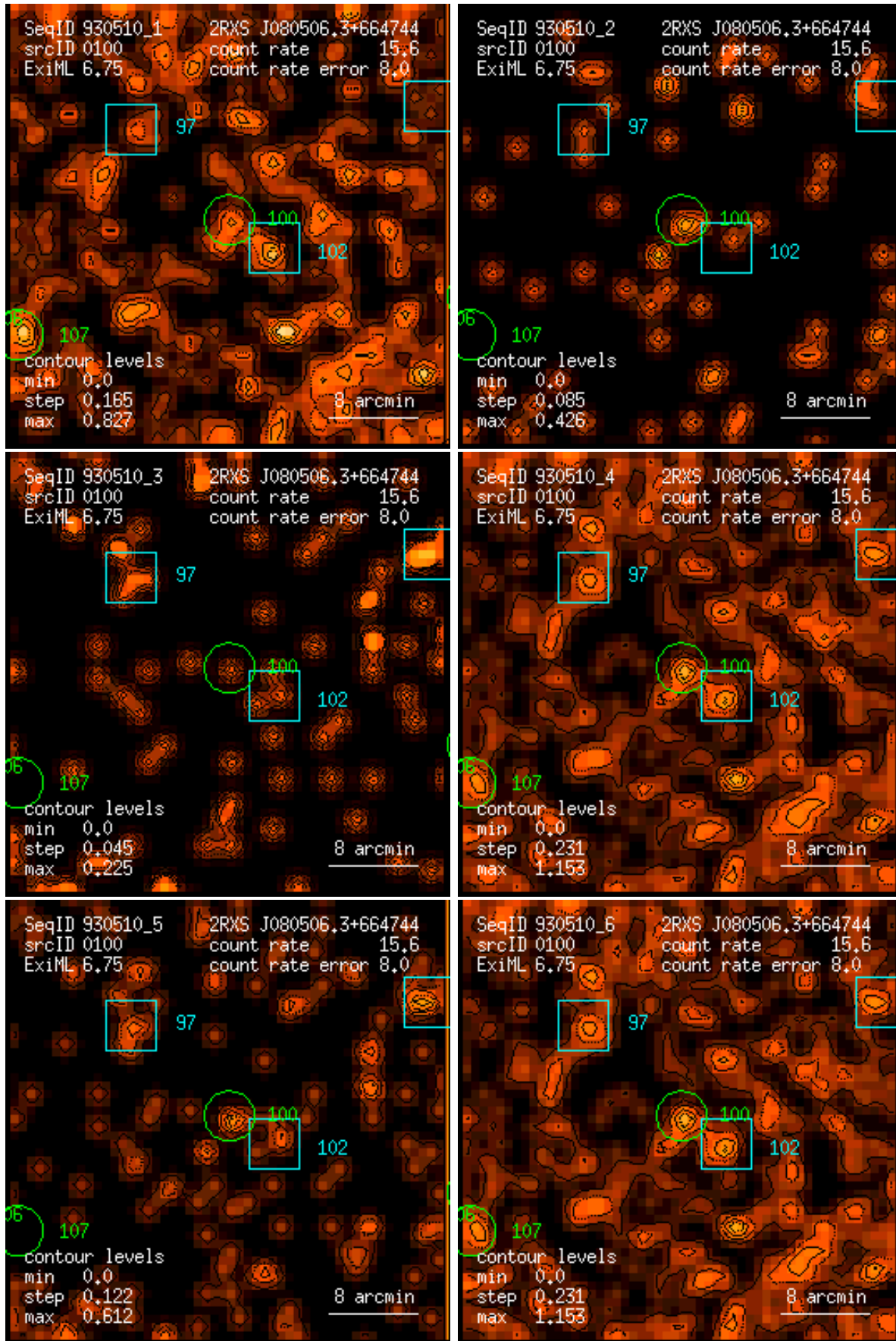
Figure 100: RASS 930510: detection 0100: band rate images, Gaussian filter: (1) PSPC channels 11 – 41, (2) 52 – 90, (3) 91 – 201, (4) 11 – 235, (5) 52 – 201, (6) 11 – 201. Broad band rates in counts/ks. Band rate contour levels in counts/ks/arcmin 2 .
