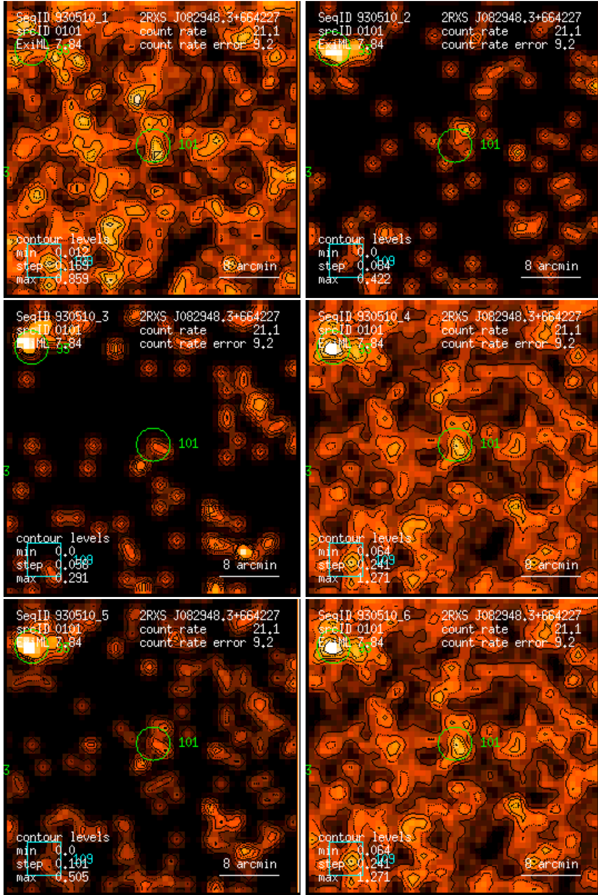
Figure 101: RASS 930510: detection 0101: band rate images, Gaussian filter: (1) PSPC channels 11 – 41, (2) 52 – 90, (3) 91 – 201, (4) 11 – 235, (5) 52 – 201, (6) 11 – 201. Broad band rates in counts/ks. Band rate contour levels in counts/ks/arcmin 2 .
