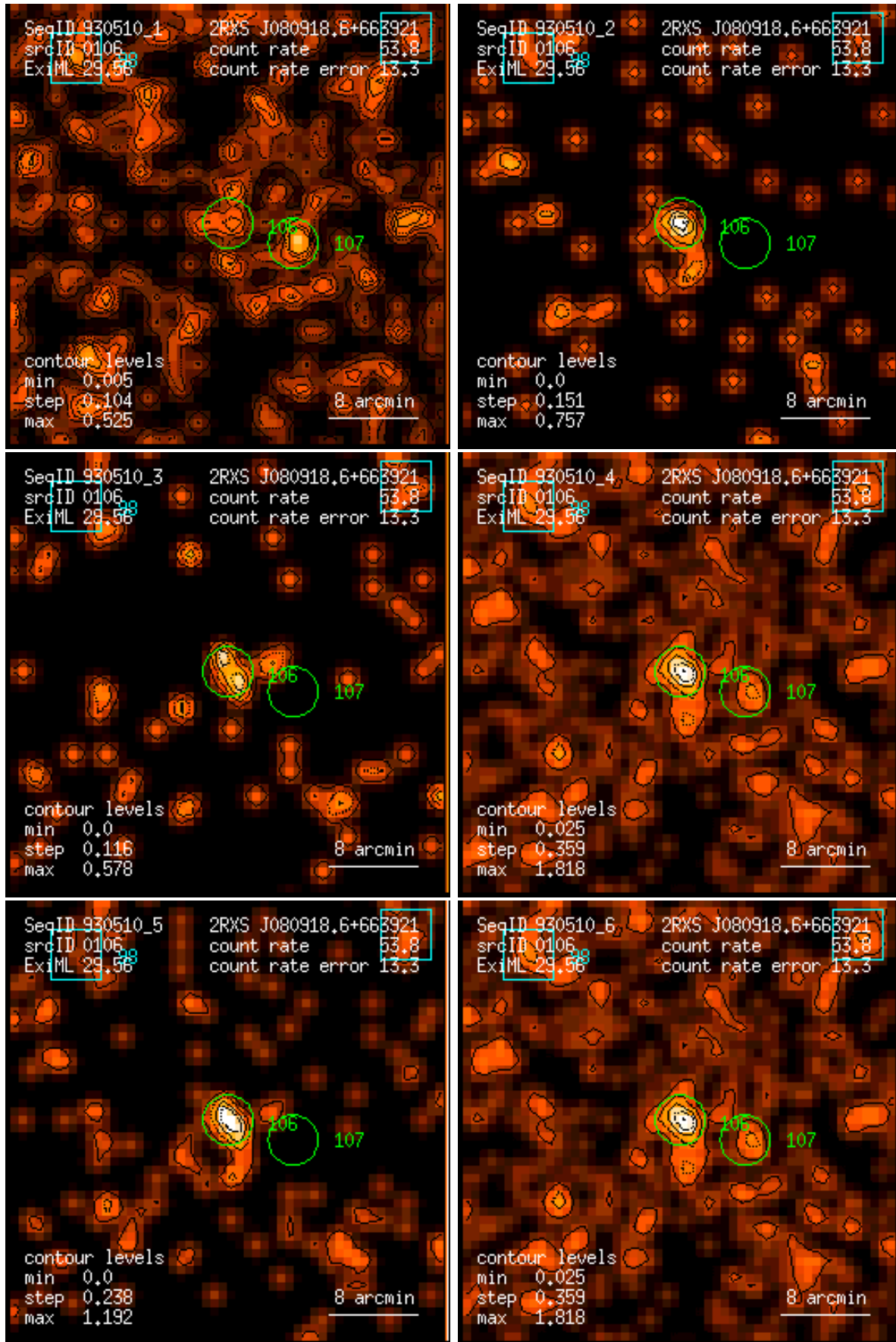
Figure 106: RASS 930510: detection 0106: band rate images, Gaussian filter: (1) PSPC channels 11 – 41, (2) 52 – 90, (3) 91 – 201, (4) 11 – 235, (5) 52 – 201, (6) 11 – 201. Broad band rates in counts/ks. Band rate contour levels in counts/ks/arcmin 2 .
