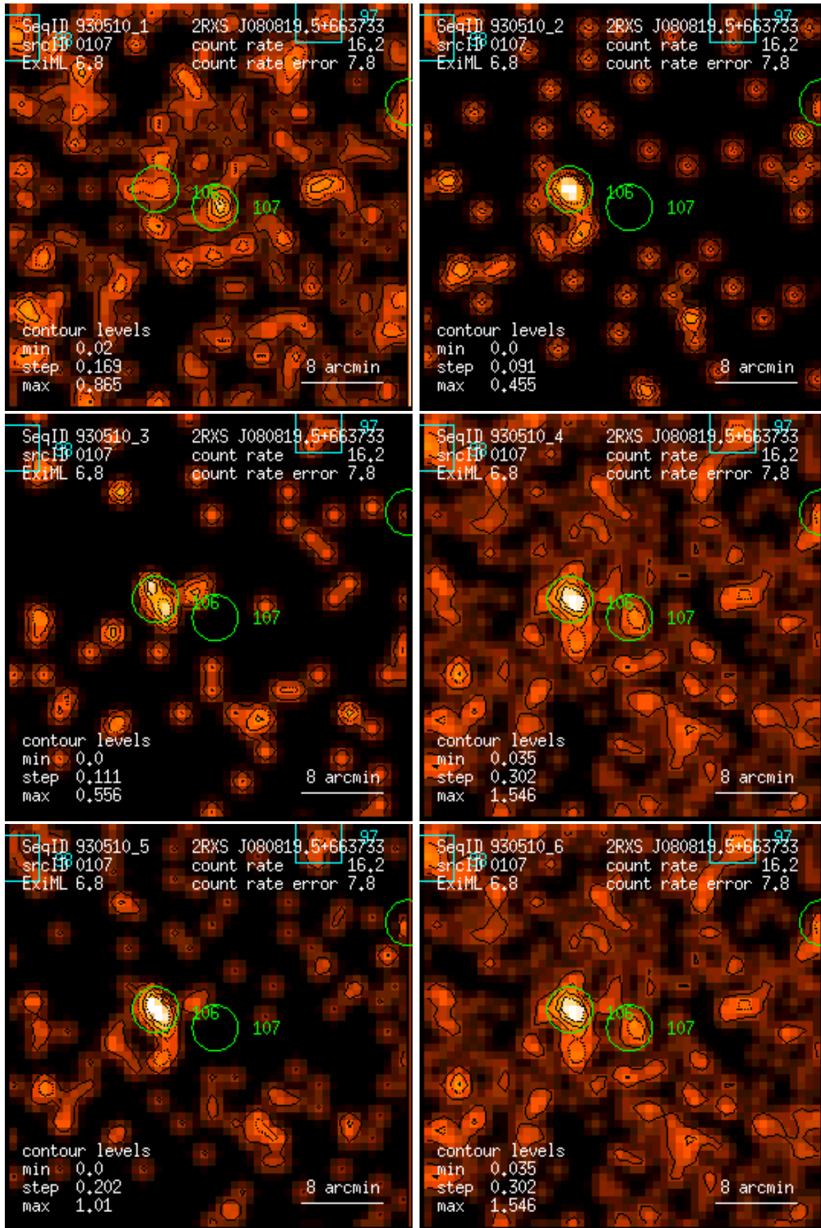
Figure 107: RASS 930510: detection 0107: band rate images, Gaussian filter: (1) PSPC channels 11 – 41, (2) 52 – 90, (3) 91 – 201, (4) 11 – 235, (5) 52 – 201, (6) 11 – 201. Broad band rates in counts/ks. Band rate contour levels in counts/ks/arcmin 2 .
