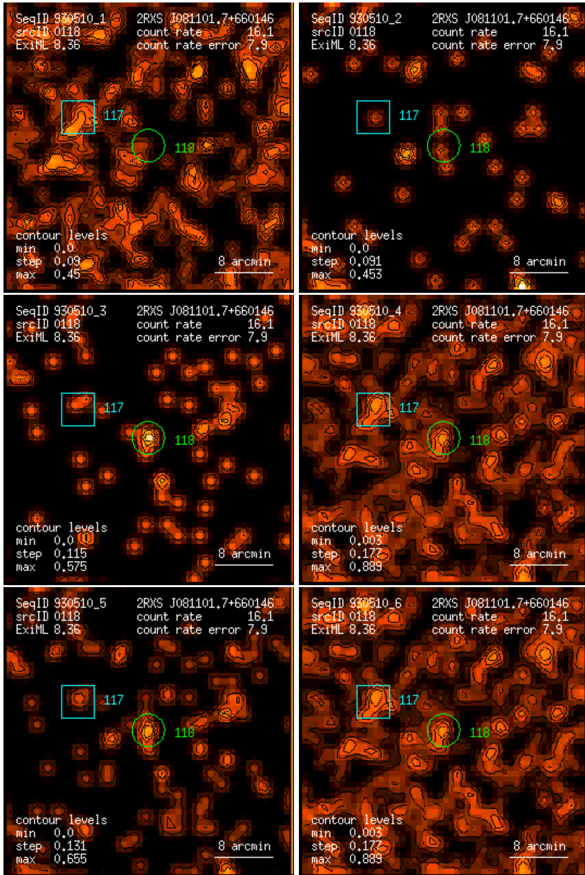
Figure 118: RASS 930510: detection 0118: band rate images, Gaussian filter: (1) PSPC channels 11 – 41, (2) 52 – 90, (3) 91 – 201, (4) 11 – 235, (5) 52 – 201, (6) 11 – 201. Broad band rates in counts/ks. Band rate contour levels in counts/ks/arcmin 2 .
