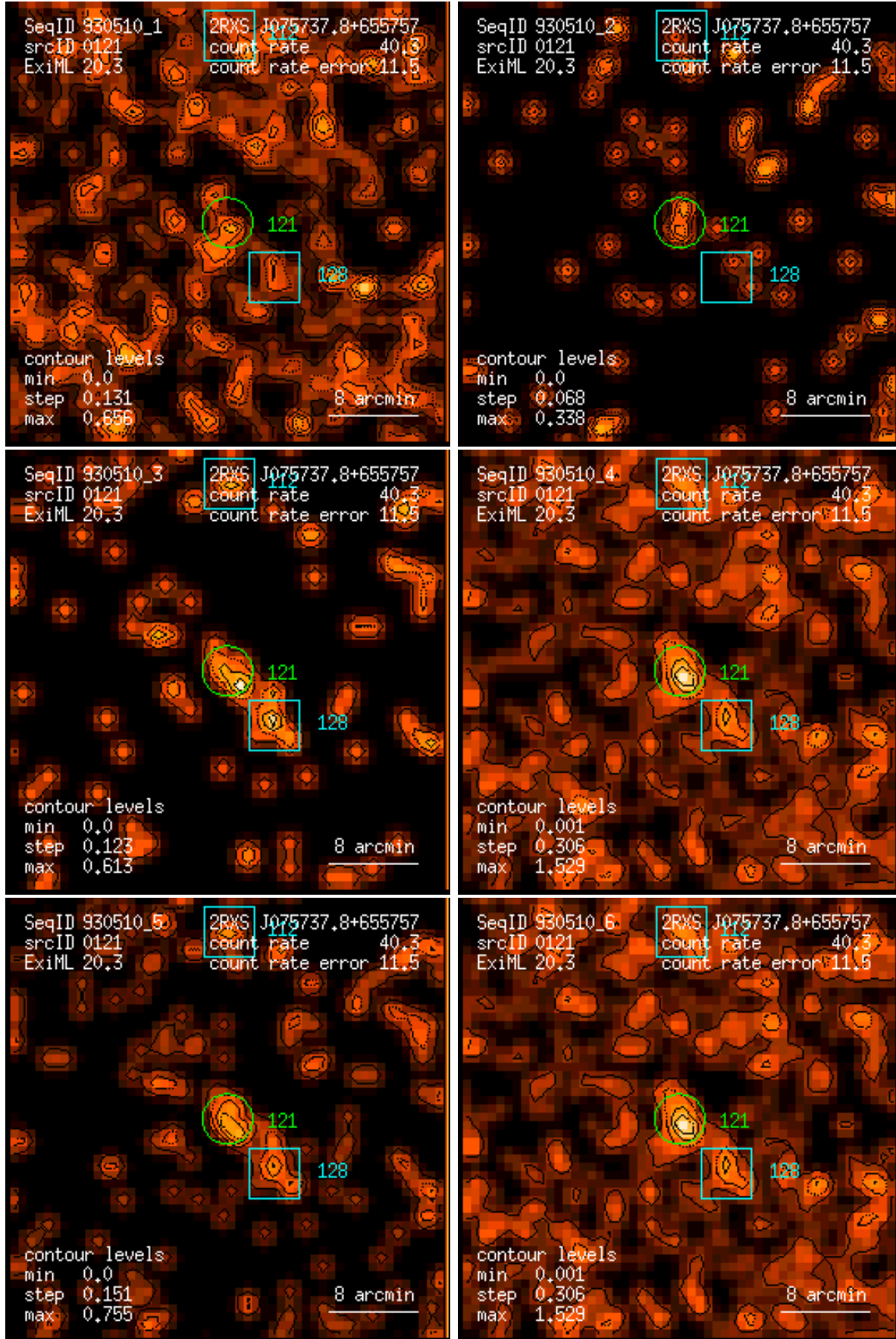
Figure 121: RASS 930510: detection 0121: band rate images, Gaussian filter: (1) PSPC channels 11 – 41, (2) 52 – 90, (3) 91 – 201, (4) 11 – 235, (5) 52 – 201, (6) 11 – 201. Broad band rates in counts/ks. Band rate contour levels in counts/ks/arcmin 2 .
