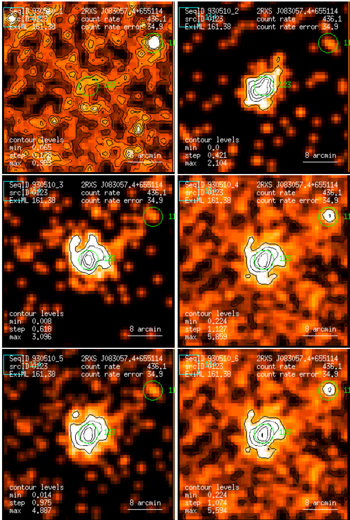
Figure 123: RASS 930510: detection 0123: band rate images, Gaussian filter: (1) PSPC channels 11 – 41, (2) 52 – 90, (3) 91 – 201, (4) 11 – 235, (5) 52 – 201, (6) 11 – 201. Broad band rates in counts/ks. Band rate contour levels in counts/ks/arcmin 2 .
