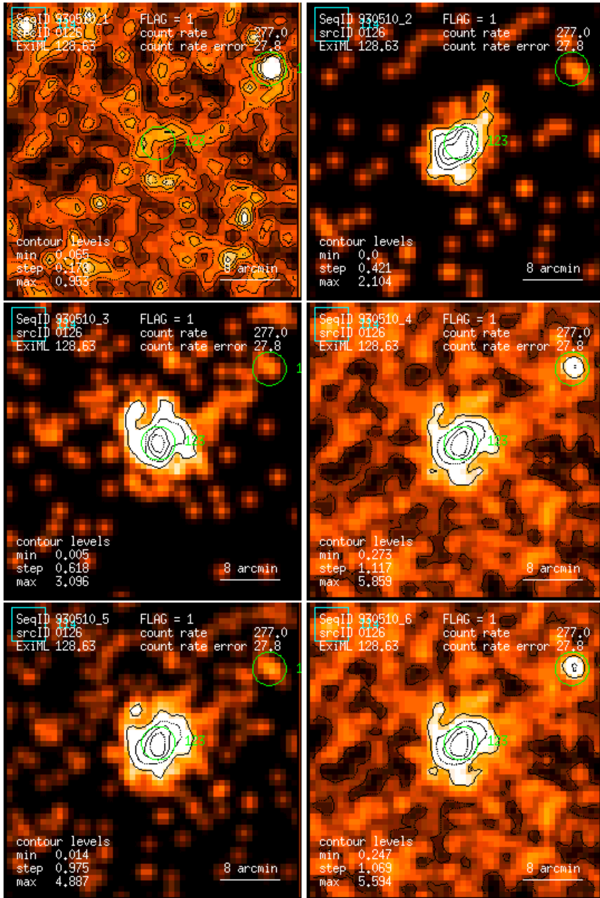
Figure 126: RASS 930510: detection 0126: band rate images, Gaussian filter: (1) PSPC channels 11 – 41, (2) 52 – 90, (3) 91 – 201, (4) 11 – 235, (5) 52 – 201, (6) 11 – 201. Broad band rates in counts/ks. Band rate contour levels in counts/ks/arcmin 2 .
