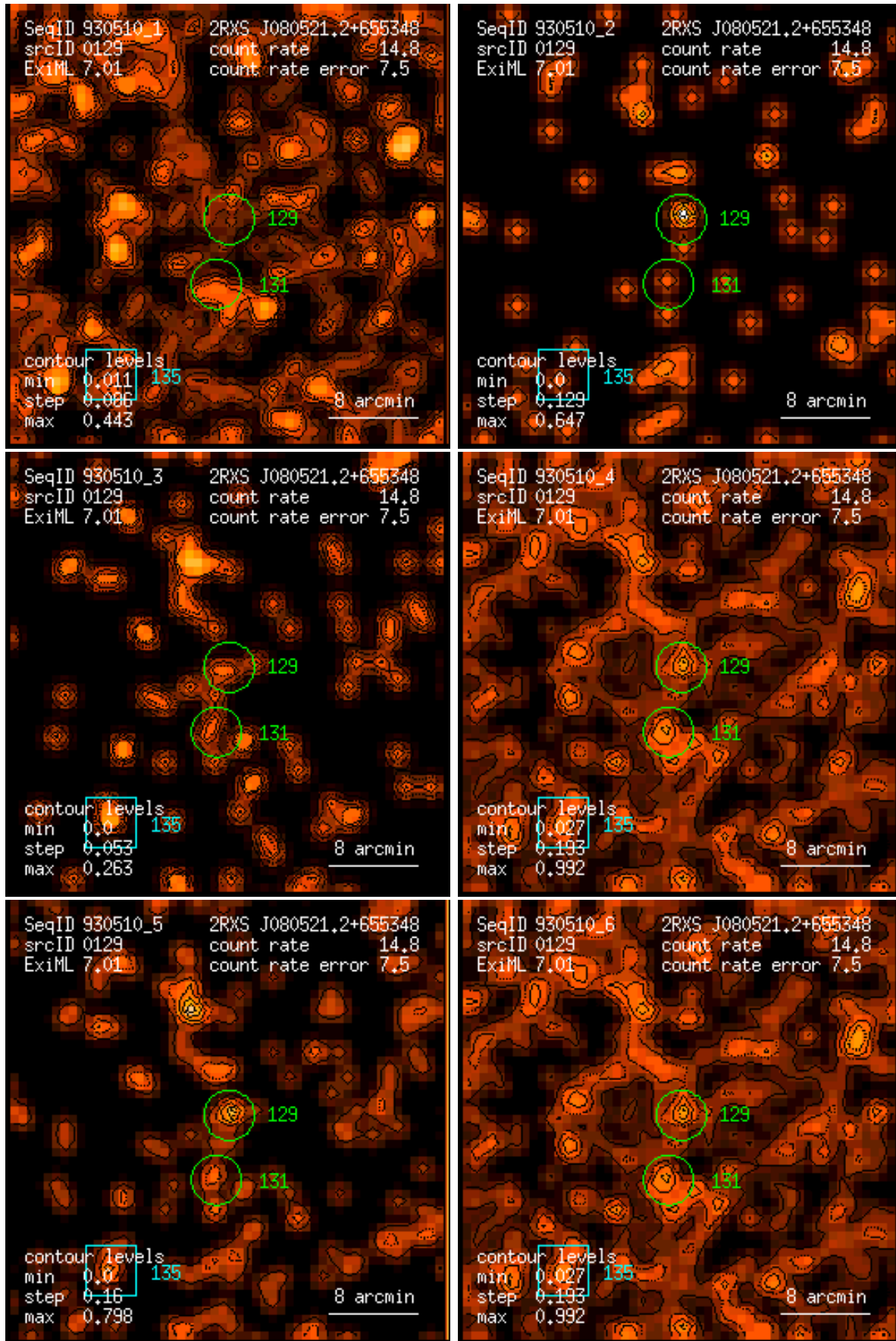
Figure 129: RASS 930510: detection 0129: band rate images, Gaussian filter: (1) PSPC channels 11 – 41, (2) 52 – 90, (3) 91 – 201, (4) 11 – 235, (5) 52 – 201, (6) 11 – 201. Broad band rates in counts/ks. Band rate contour levels in counts/ks/arcmin 2 .
