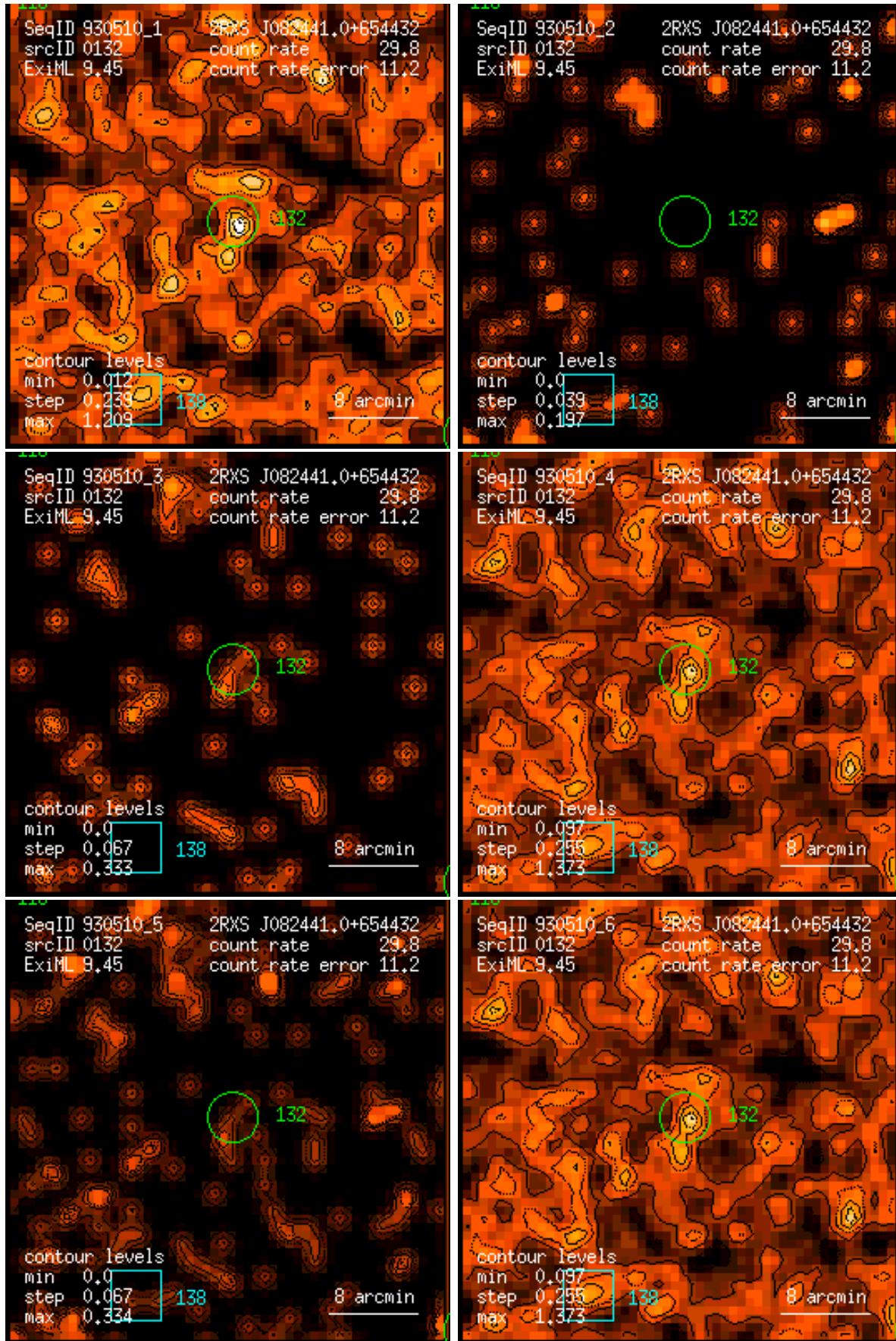
Figure 132: RASS 930510: detection 0132: band rate images, Gaussian filter: (1) PSPC channels 11 – 41, (2) 52 – 90, (3) 91 – 201, (4) 11 – 235, (5) 52 – 201, (6) 11 – 201. Broad band rates in counts/ks. Band rate contour levels in counts/ks/arcmin 2 .
