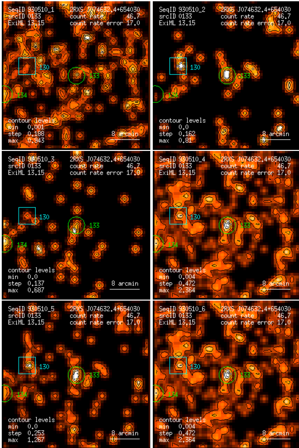
Figure 133: RASS 930510: detection 0133: band rate images, Gaussian filter: (1) PSPC channels 11 – 41, (2) 52 – 90, (3) 91 – 201, (4) 11 – 235, (5) 52 – 201, (6) 11 – 201. Broad band rates in counts/ks. Band rate contour levels in counts/ks/arcmin 2 .
