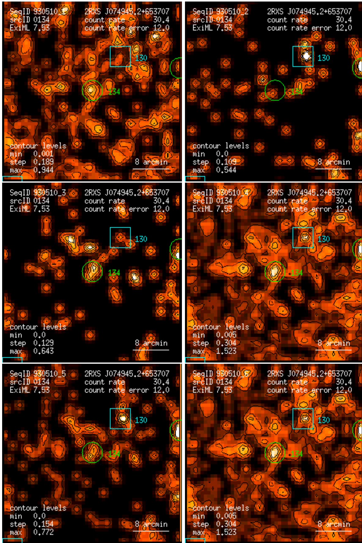
Figure 134: RASS 930510: detection 0134: band rate images, Gaussian filter: (1) PSPC channels 11 – 41, (2) 52 – 90, (3) 91 – 201, (4) 11 – 235, (5) 52 – 201, (6) 11 – 201. Broad band rates in counts/ks. Band rate contour levels in counts/ks/arcmin 2 .
