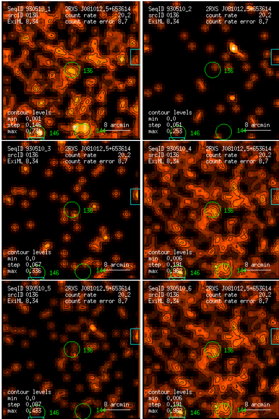
Figure 136: RASS 930510: detection 0136: band rate images, Gaussian filter: (1) PSPC channels 11 – 41, (2) 52 – 90, (3) 91 – 201, (4) 11 – 235, (5) 52 – 201, (6) 11 – 201. Broad band rates in counts/ks. Band rate contour levels in counts/ks/arcmin 2 .
