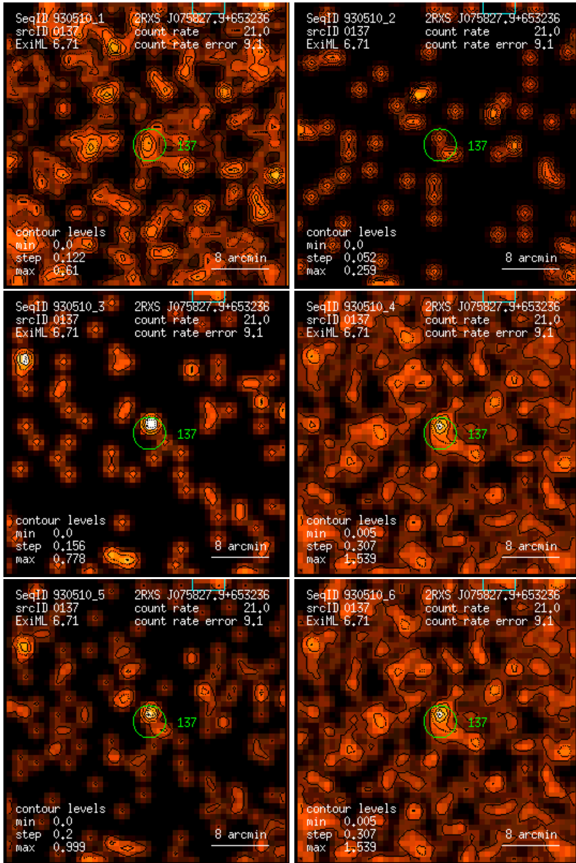
Figure 137: RASS 930510: detection 0137: band rate images, Gaussian filter: (1) PSPC channels 11 – 41, (2) 52 – 90, (3) 91 – 201, (4) 11 – 235, (5) 52 – 201, (6) 11 – 201. Broad band rates in counts/ks. Band rate contour levels in counts/ks/arcmin 2 .
